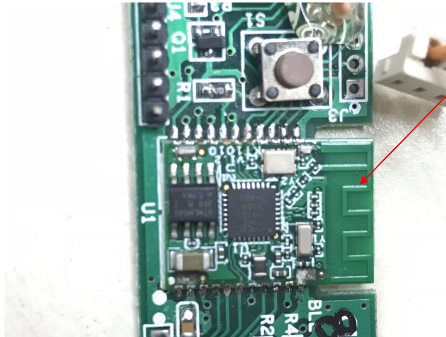
RF Antenna
