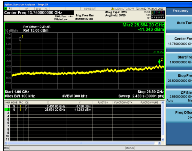
3DH5-Ant1-2441-0~Reference--3.40
