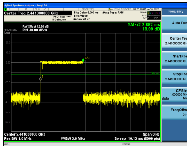
2DH1-Ant1-Hop-0.390-320
