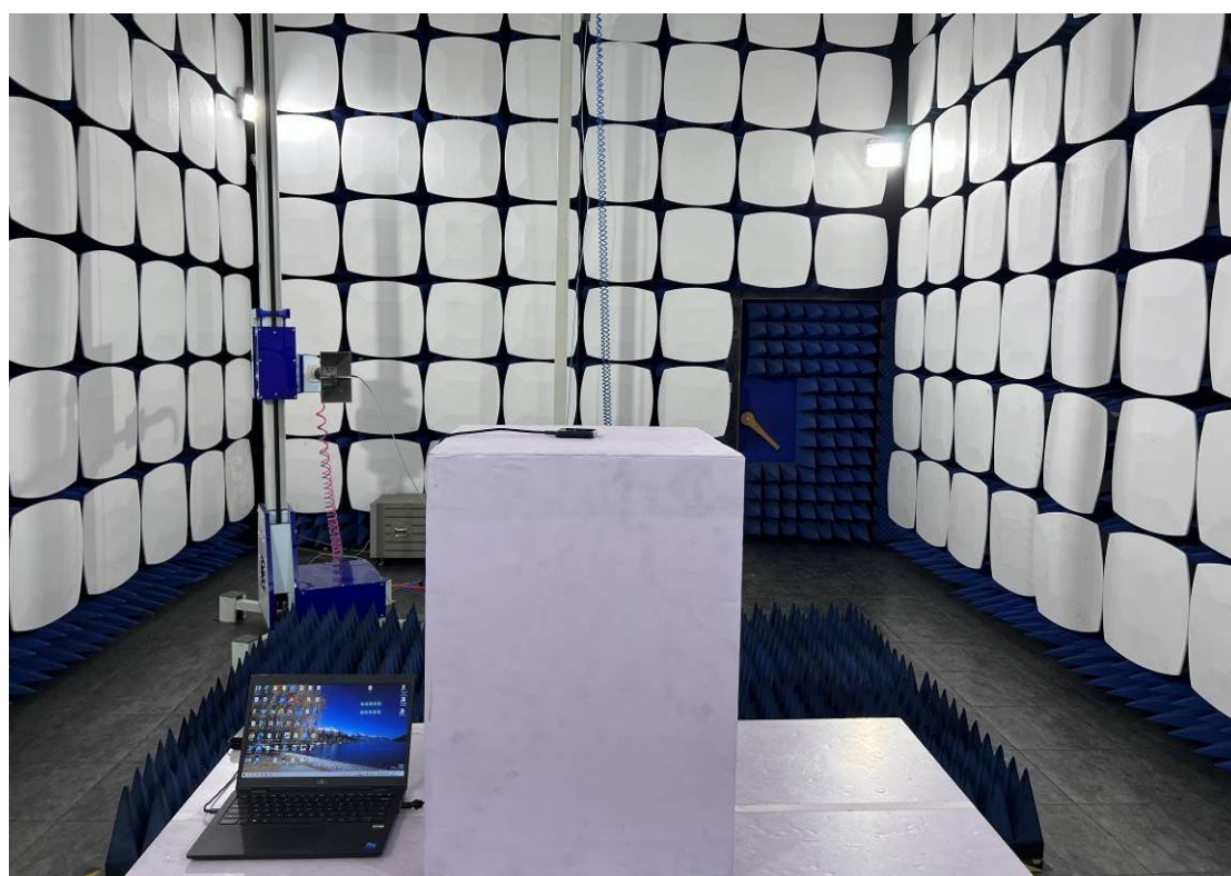
6. RF measurement setup
