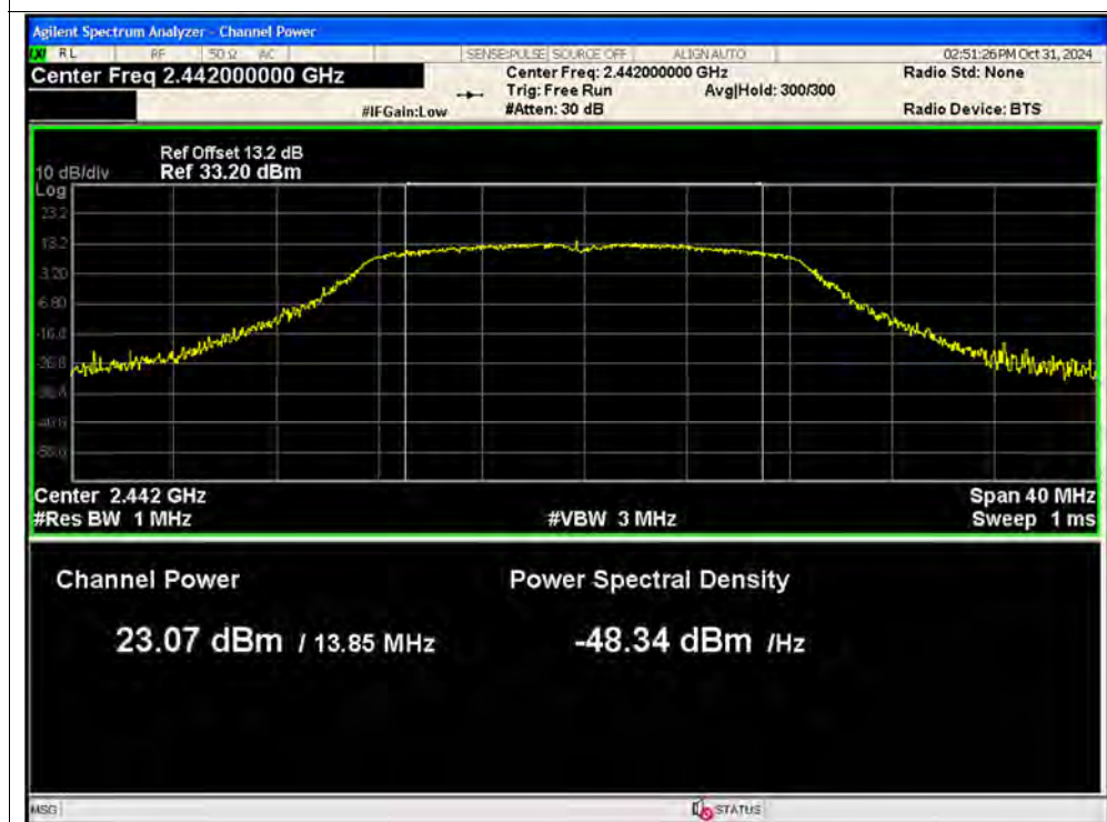
Peak Power NVNT n20 2442MHz Ant1
