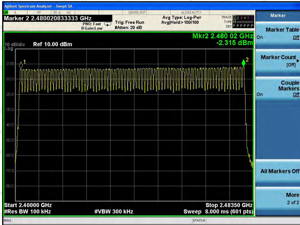
GFSK Mode
