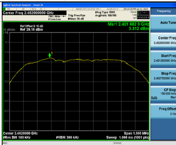
\pi/4 -DQPSK on Channel 00
