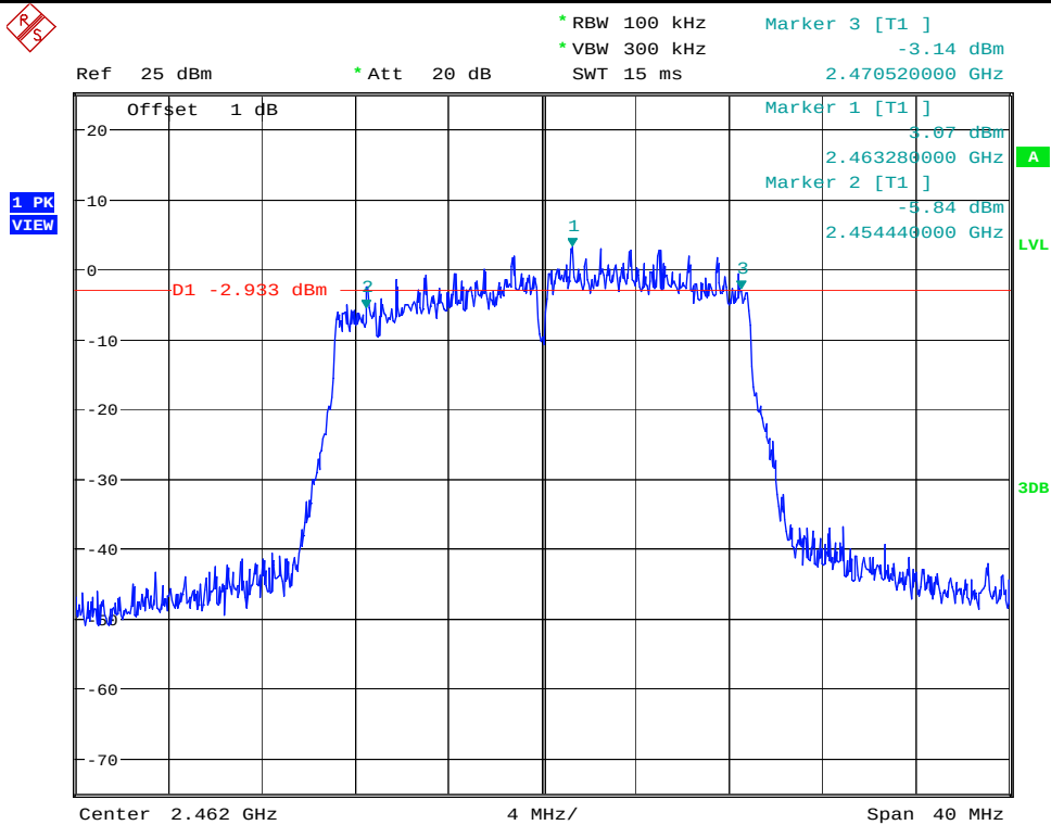
6dB Bandwidth_11N20SISO_2462_Ant1
