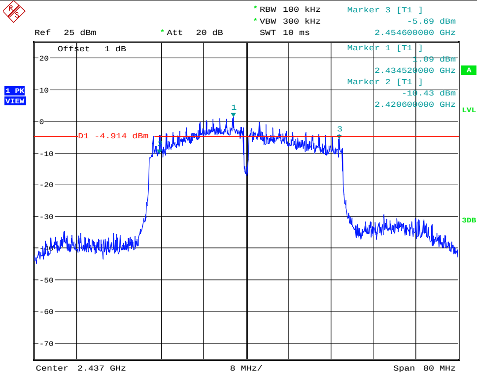
6dB Bandwidth_11N40SISO_2437_Ant1
