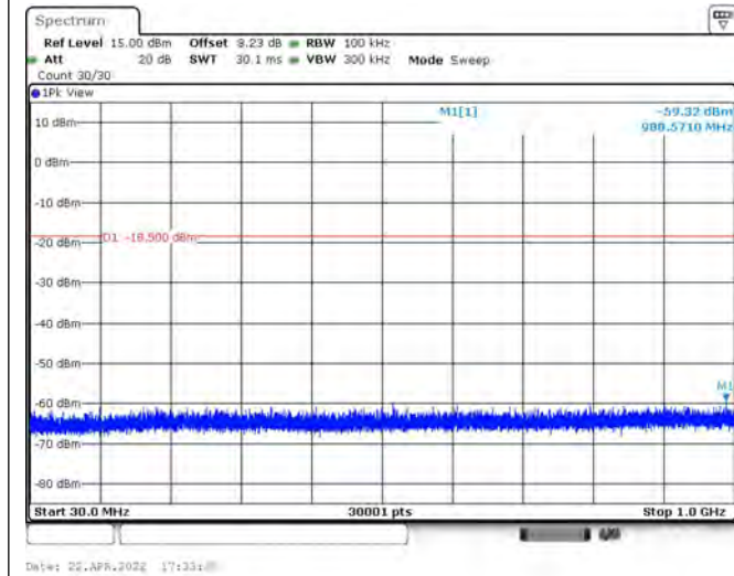
GFSK 1M
