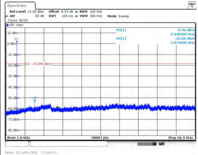
GFSK 1M
