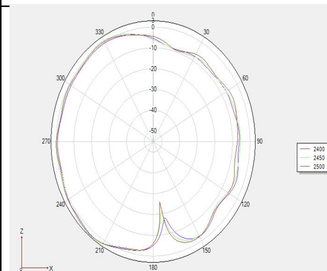
Phi 0 2D
