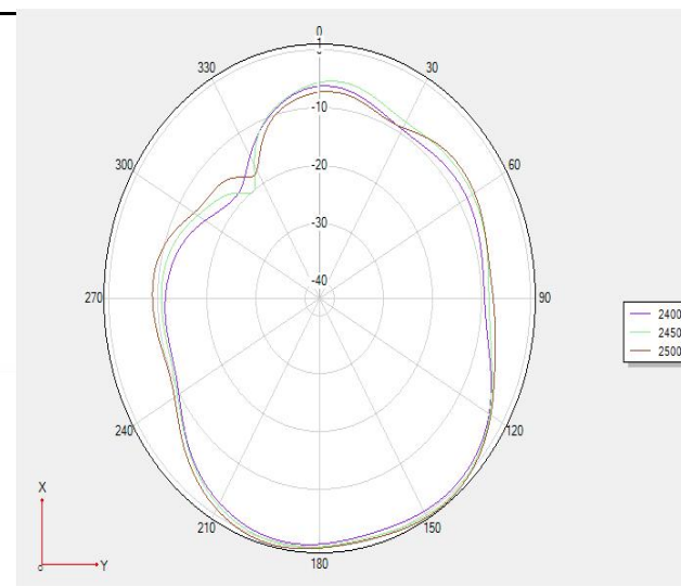
Theta 90 2D
