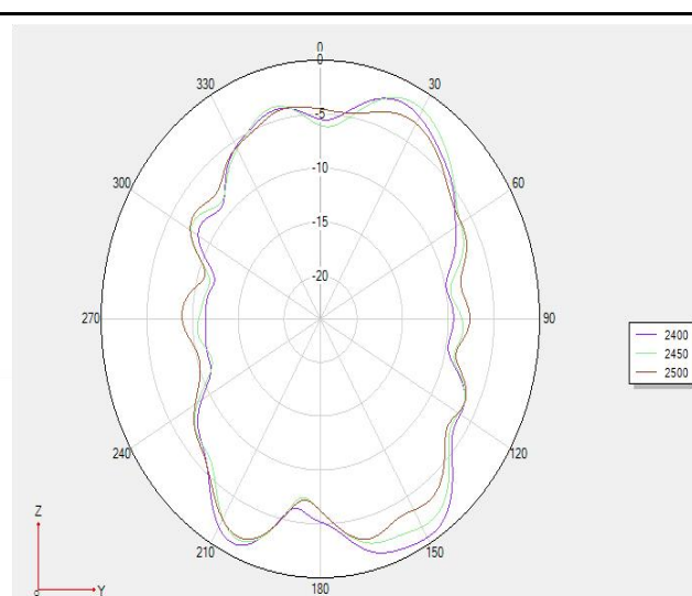
Phi 90 2D
