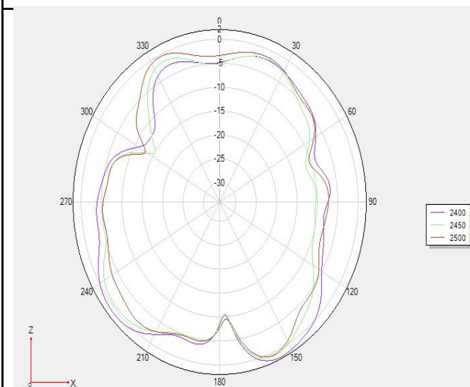
Phi 0 2D
