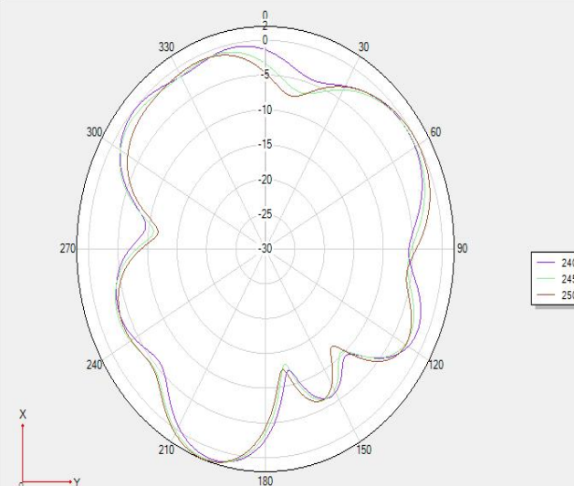
Theta 90 2D
