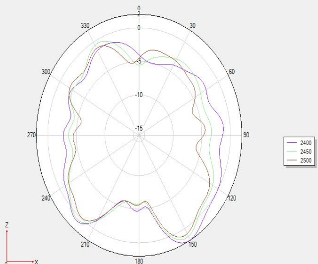
Phi 0 2D
