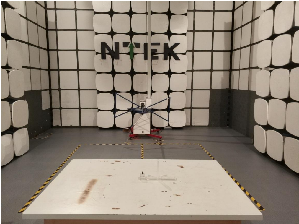
Radiated Measurement Photos (Right)
