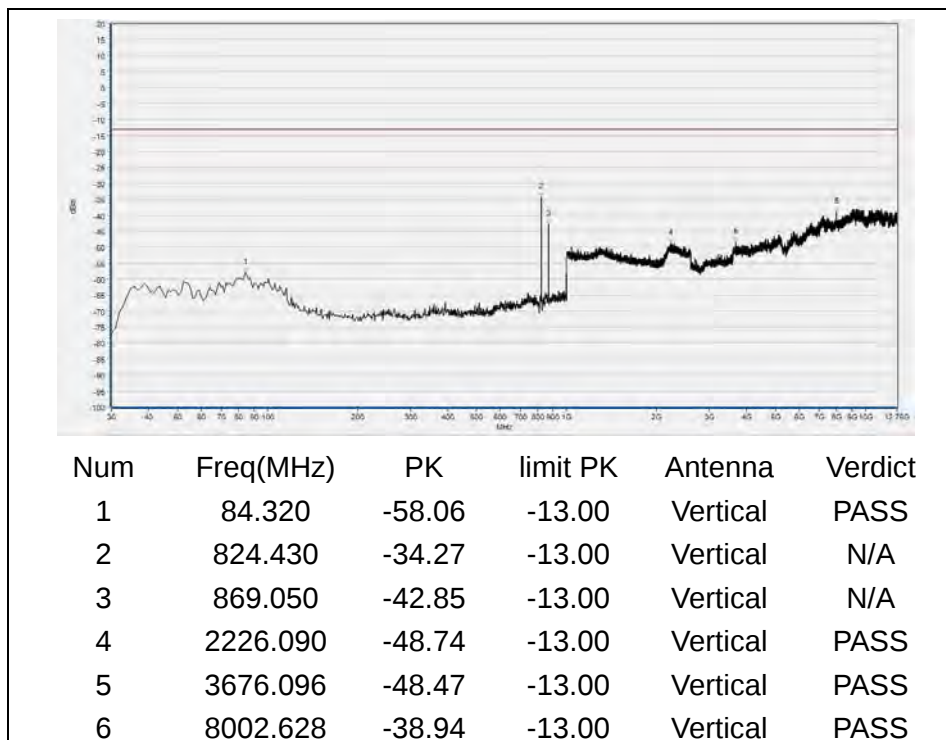
(Plot A2, GSM 850MHz, Channel = 128, Vertical)
