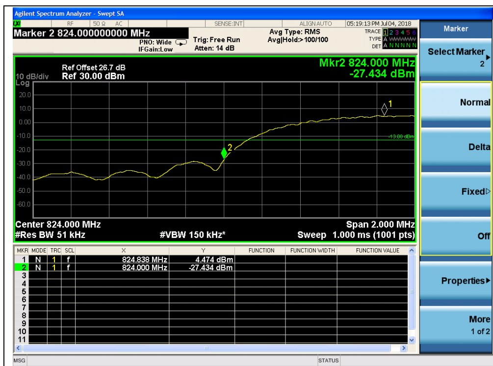
(Plot K1, HSUPA 850, Channel = 4132)
