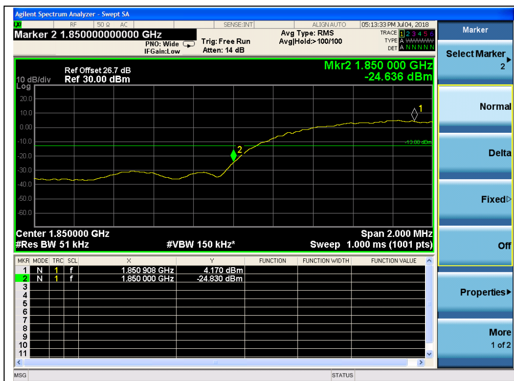
(Plot J1, HSDPA 1900, Channel = 9262)
