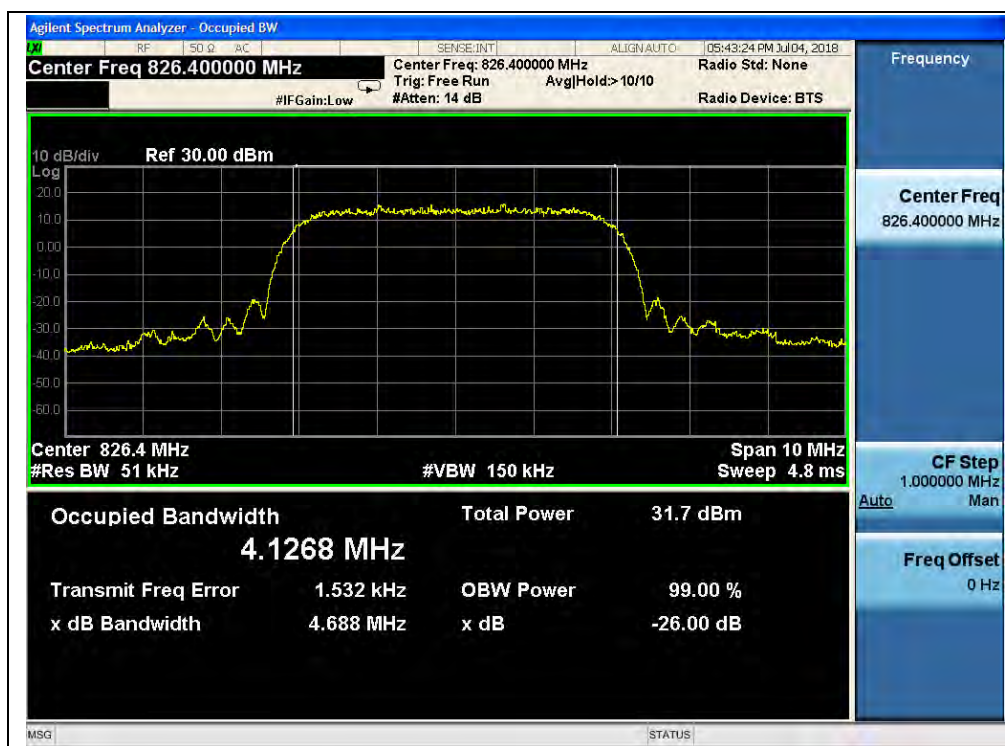
(Plot P1, HSPA+ 850MHz, Channel = 4132)
