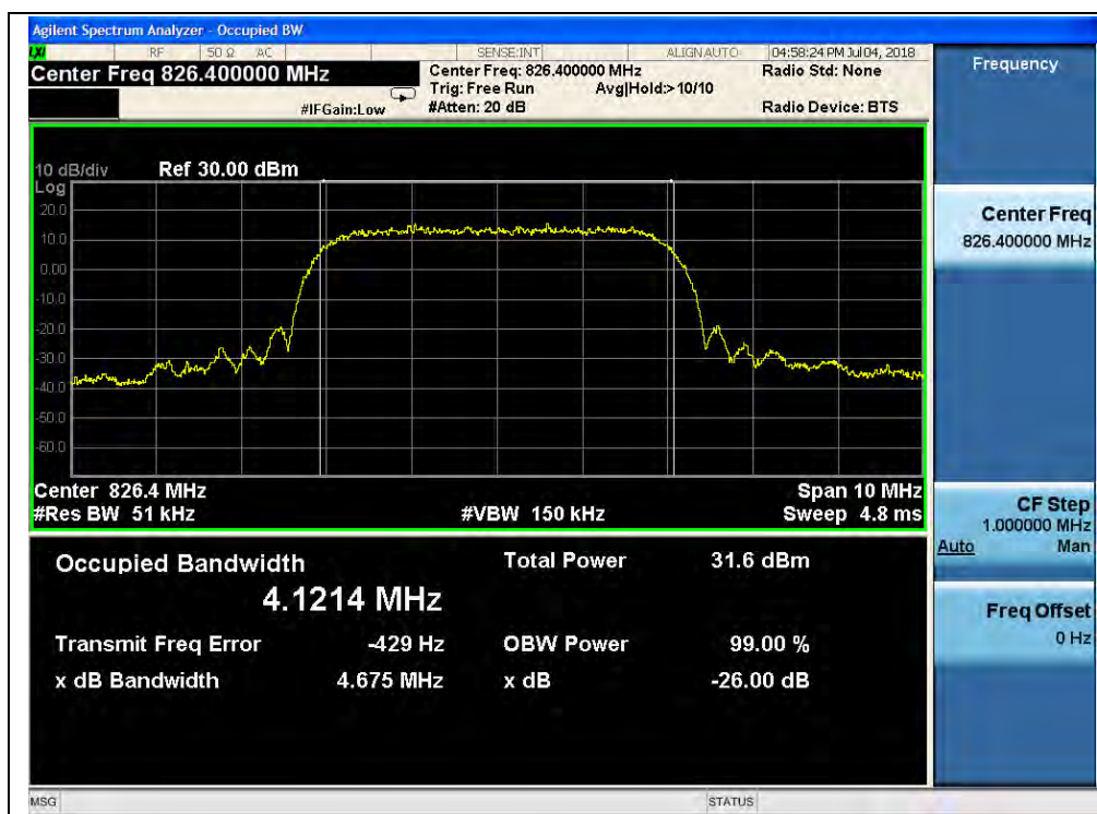
(Plot J1, HSDPA 850MHz, Channel = 4132)
