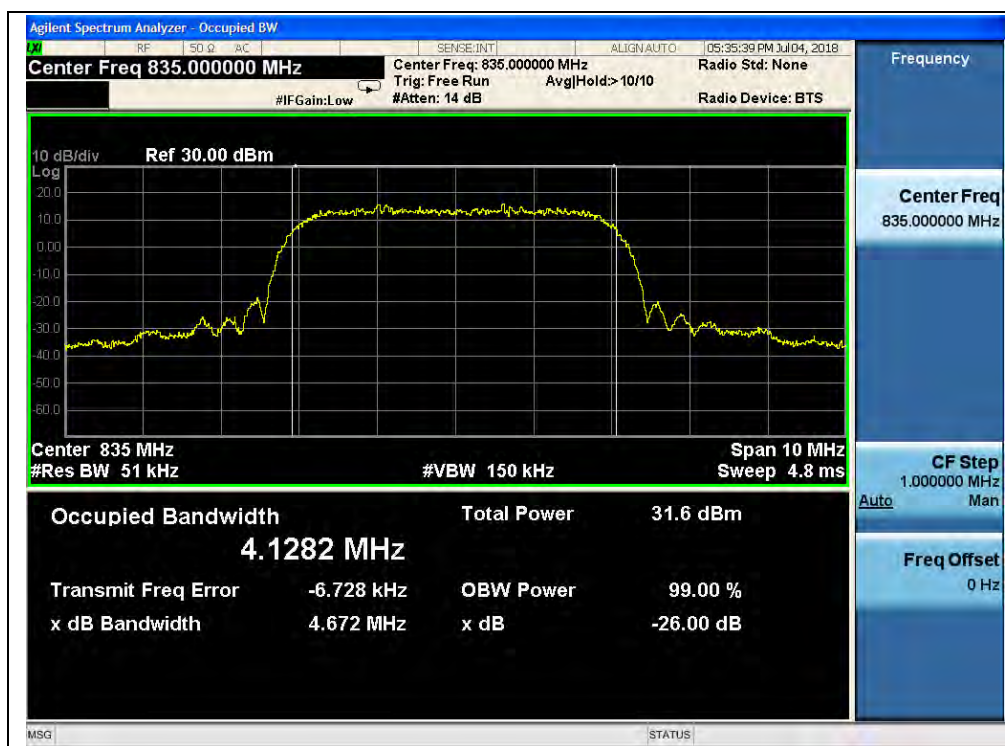
(Plot M2, HSUPA 850 MHz, Channel = 4175)
