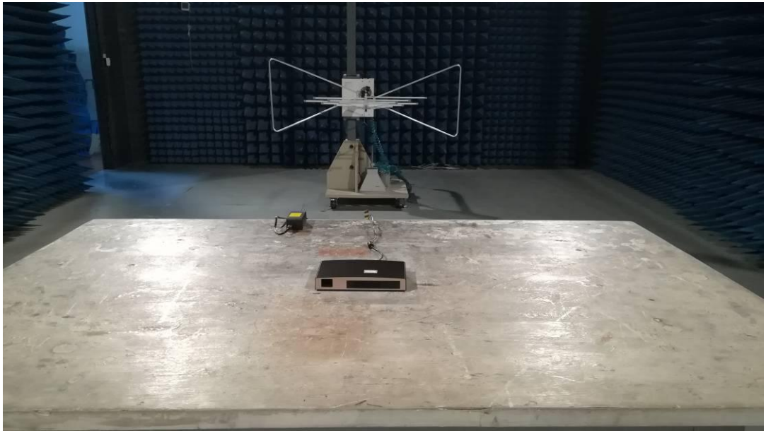
Radiated Emission
