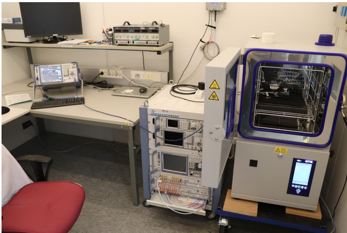
Photograph 4: Test setup for Frequency Stability and Occupied Bandwidth
