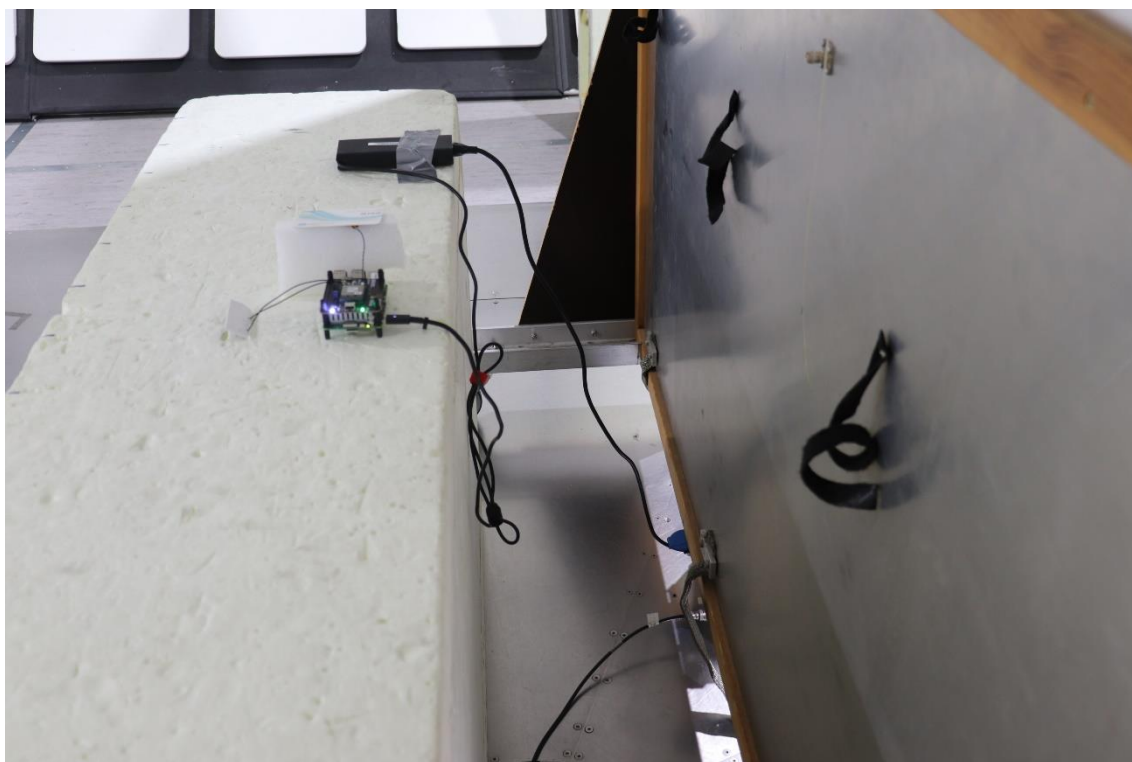
Photograph 6: Test setup for AC Power-Line Conducted Emissions
