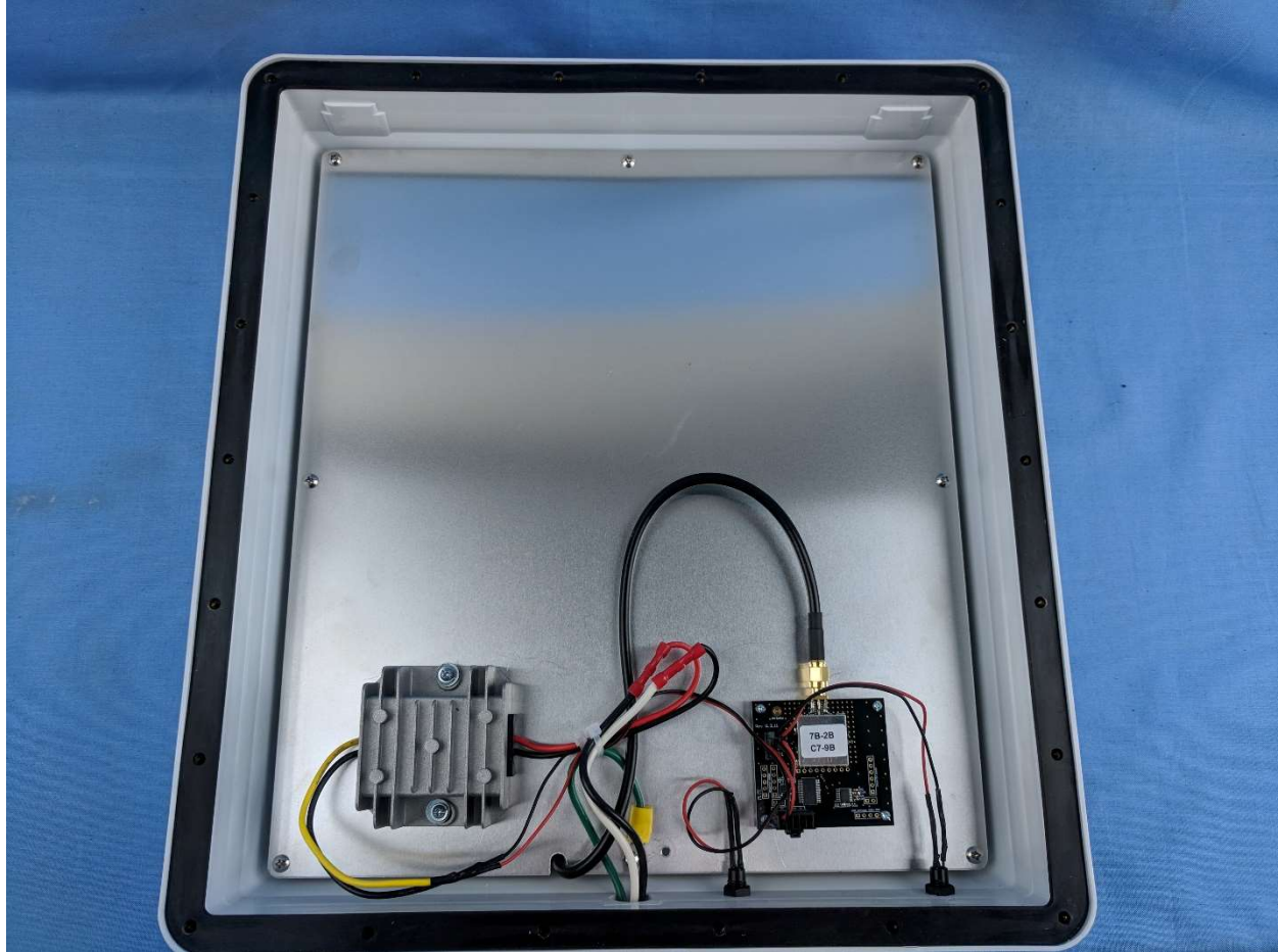
DV21DC Internal
