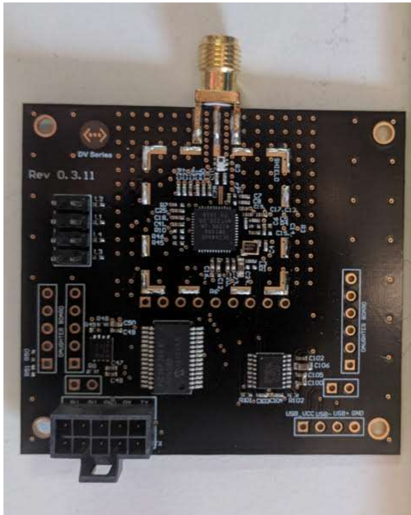
Module top – shield removed
