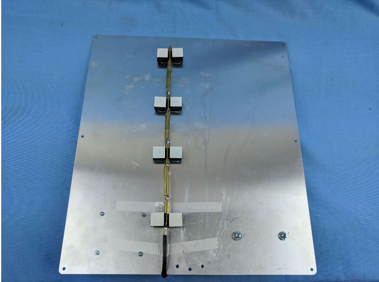
DV21AC Antenna
