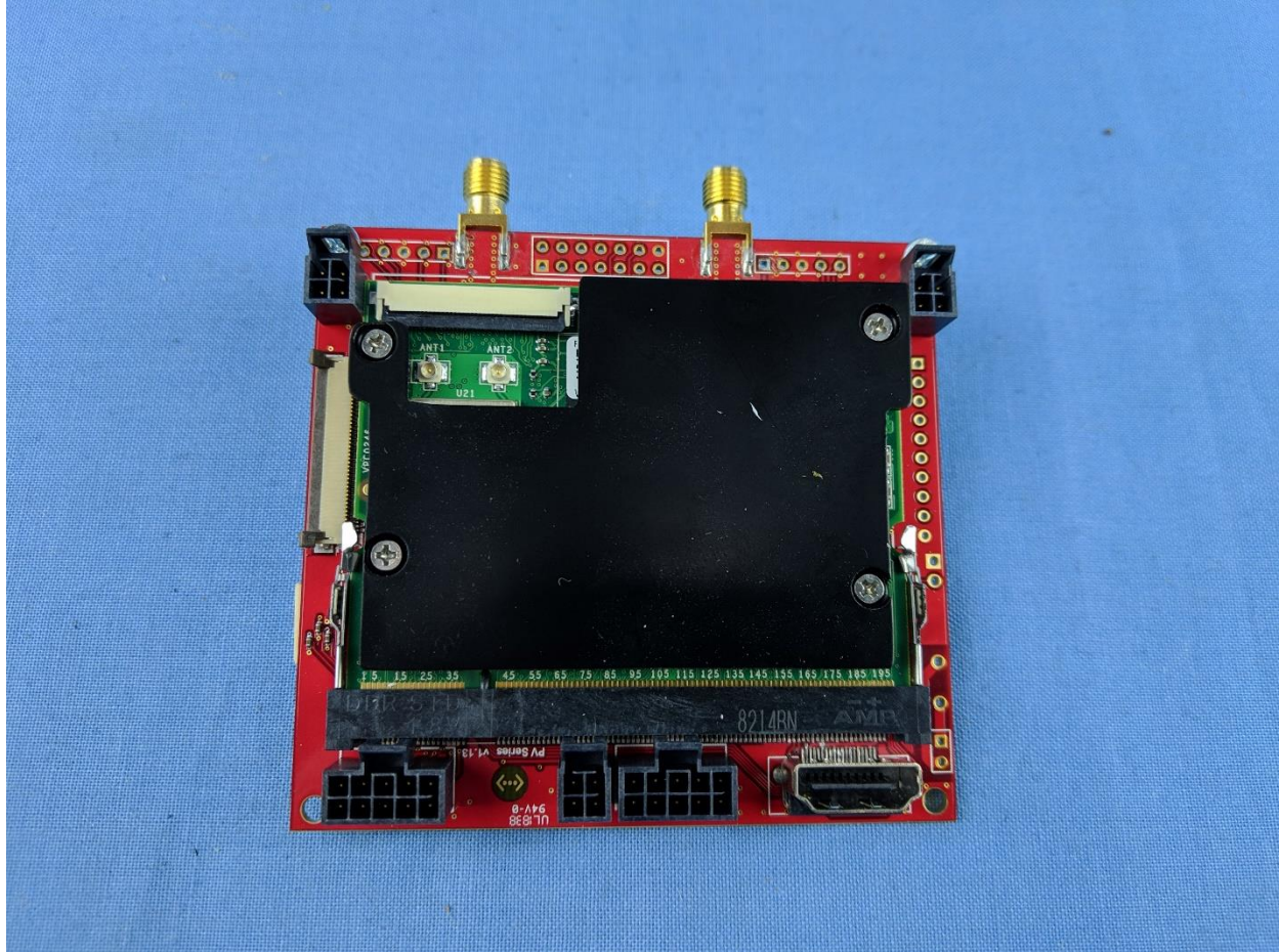
IO Board Top View
