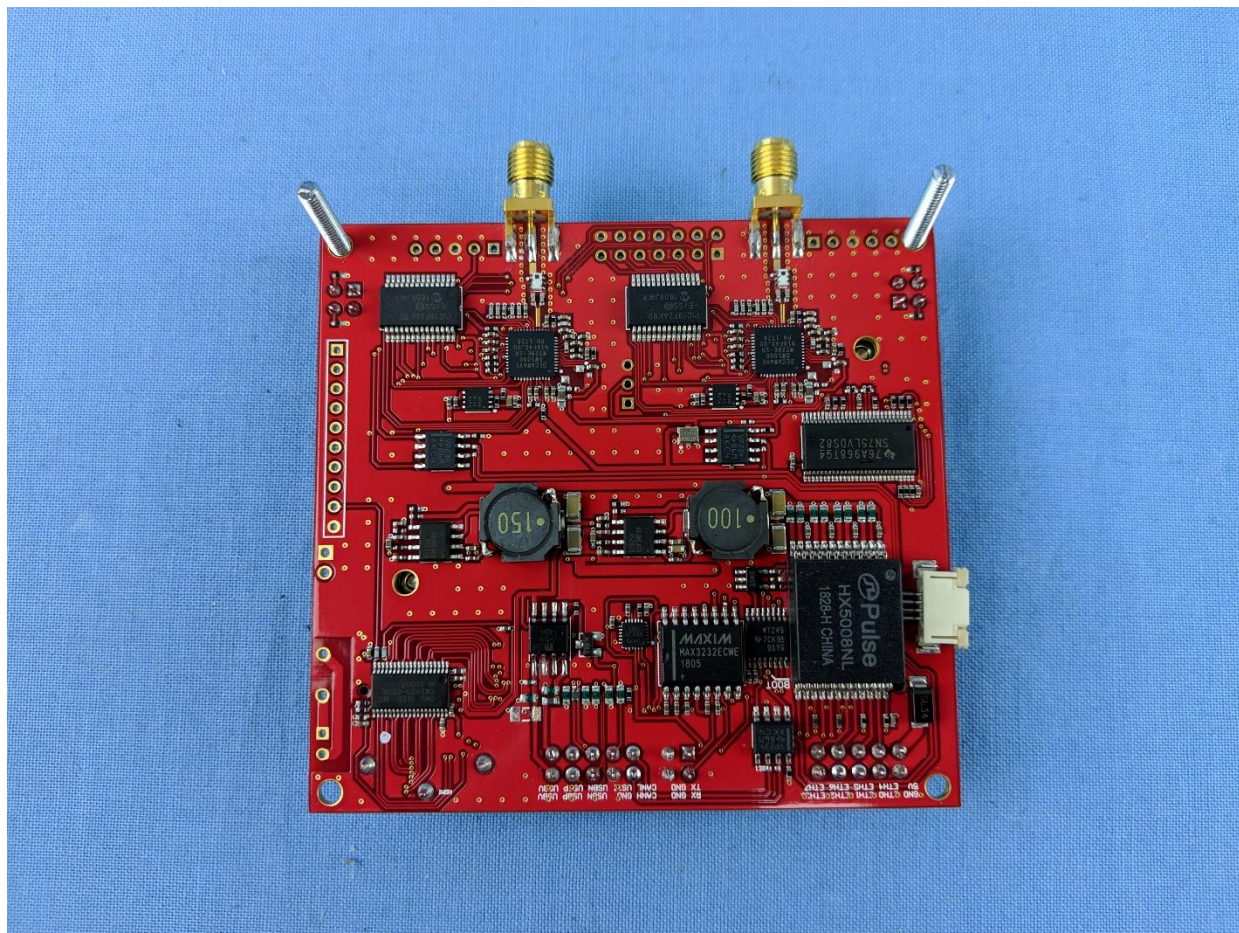
IO Board Bottom View
