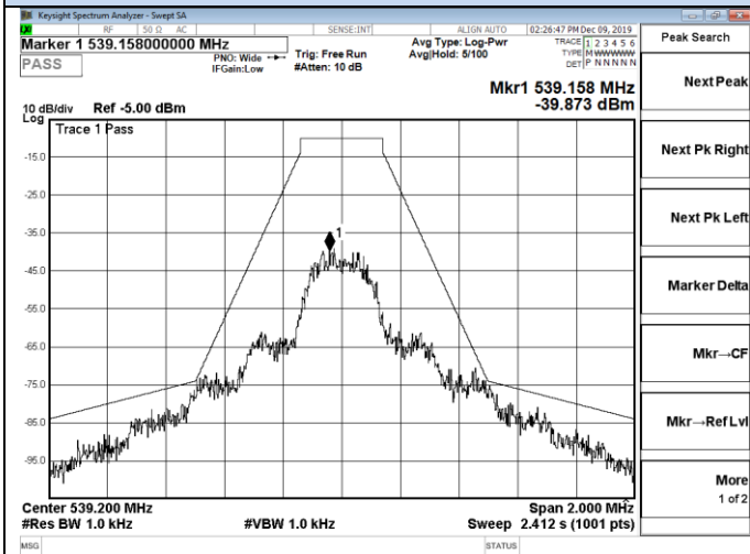
Channel 60 / 539.2MHz
