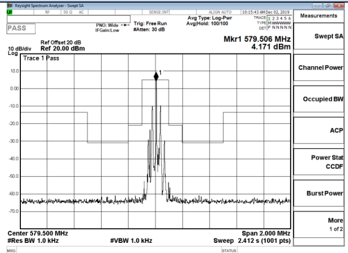
Channel 22 / 579.5 MHz
