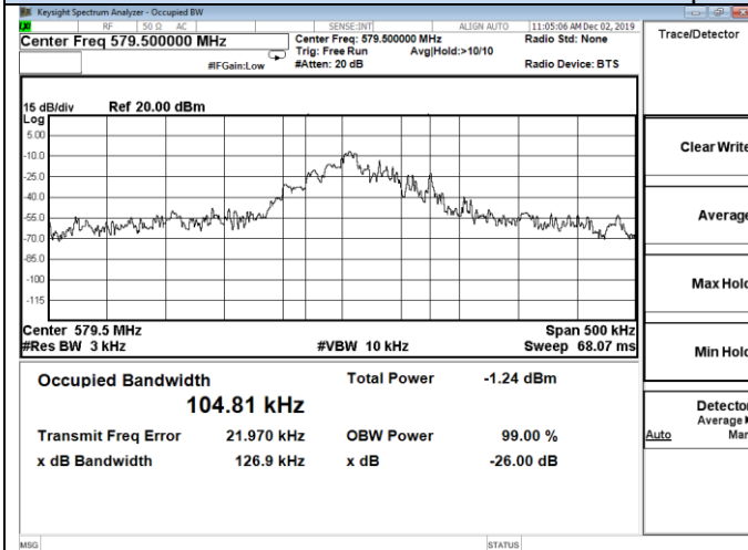
Channel 22 / 579.5 MHz
