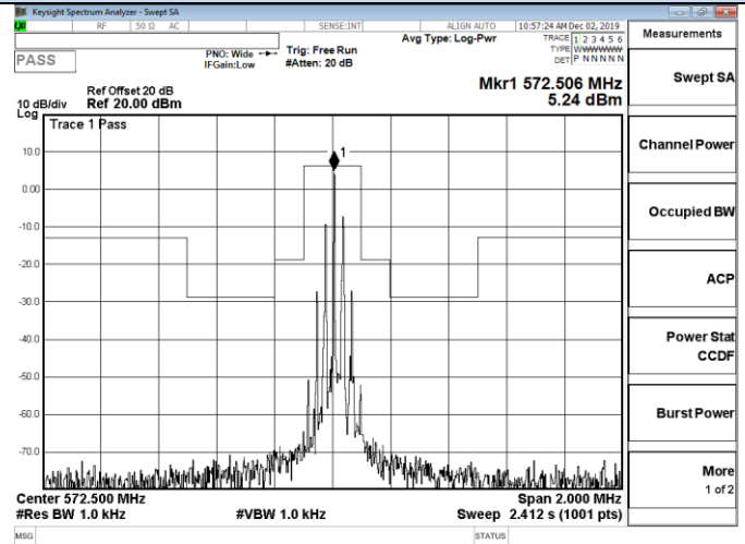
Channel 15 / 572.5MHz
