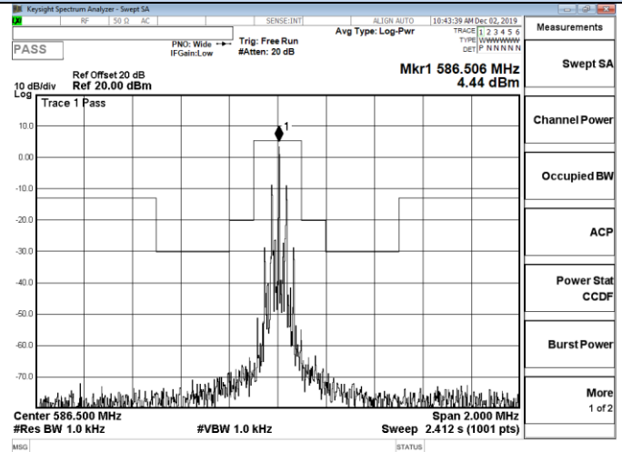
Channel 29 / 586.5 MHz
