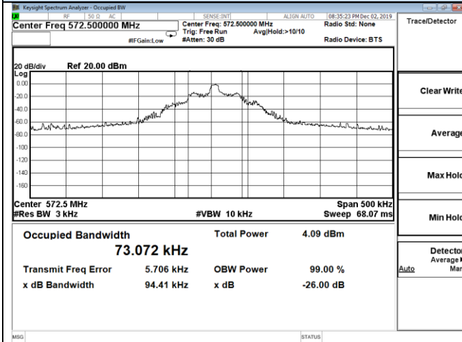
Channel 15 / 572.5MHz
