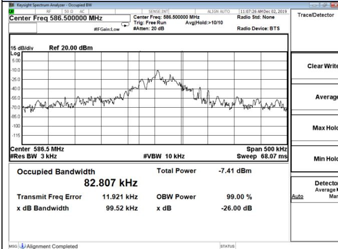
Channel 29 / 586.5 MHz
