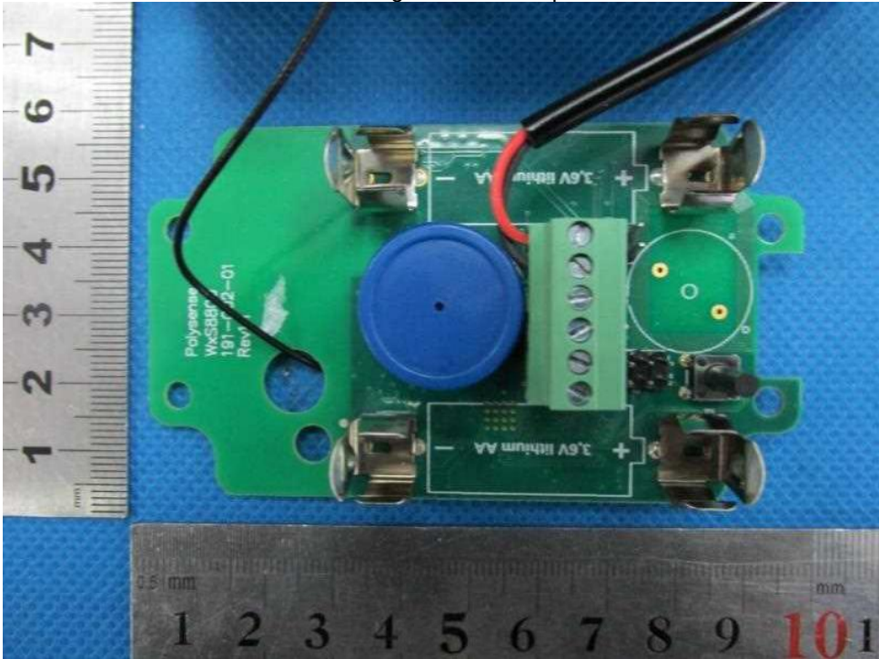
Alternative configuration for Whip antenna
