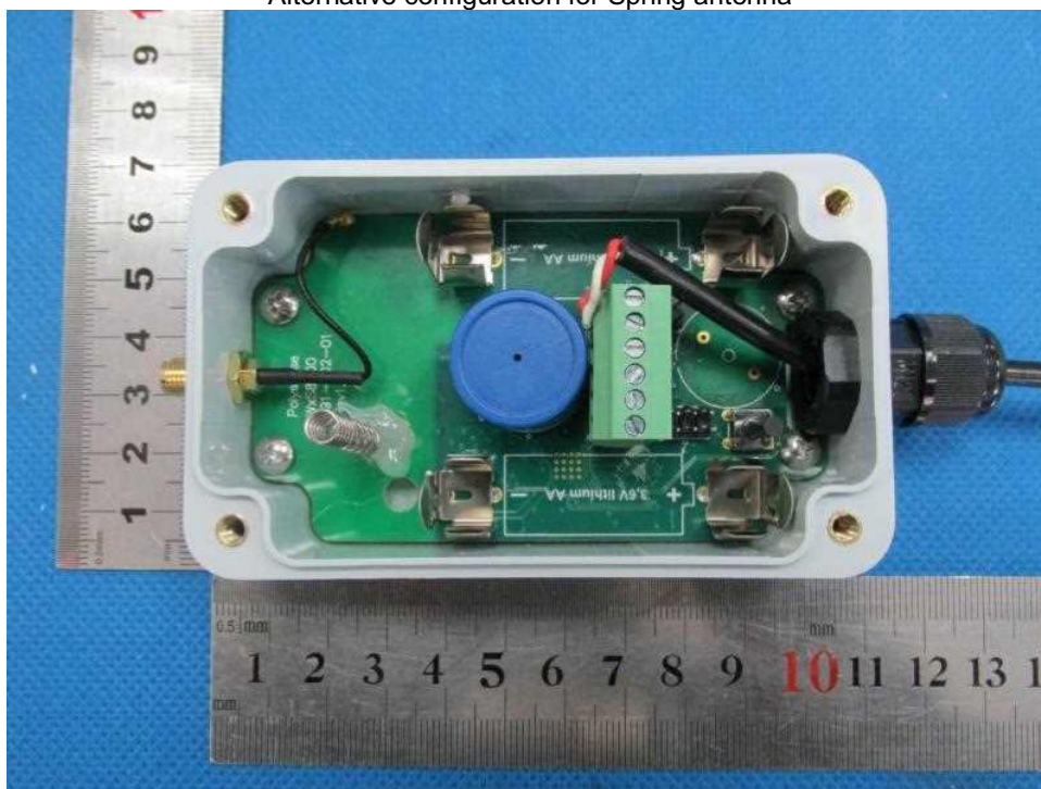
Alternative configuration for Spring antenna
