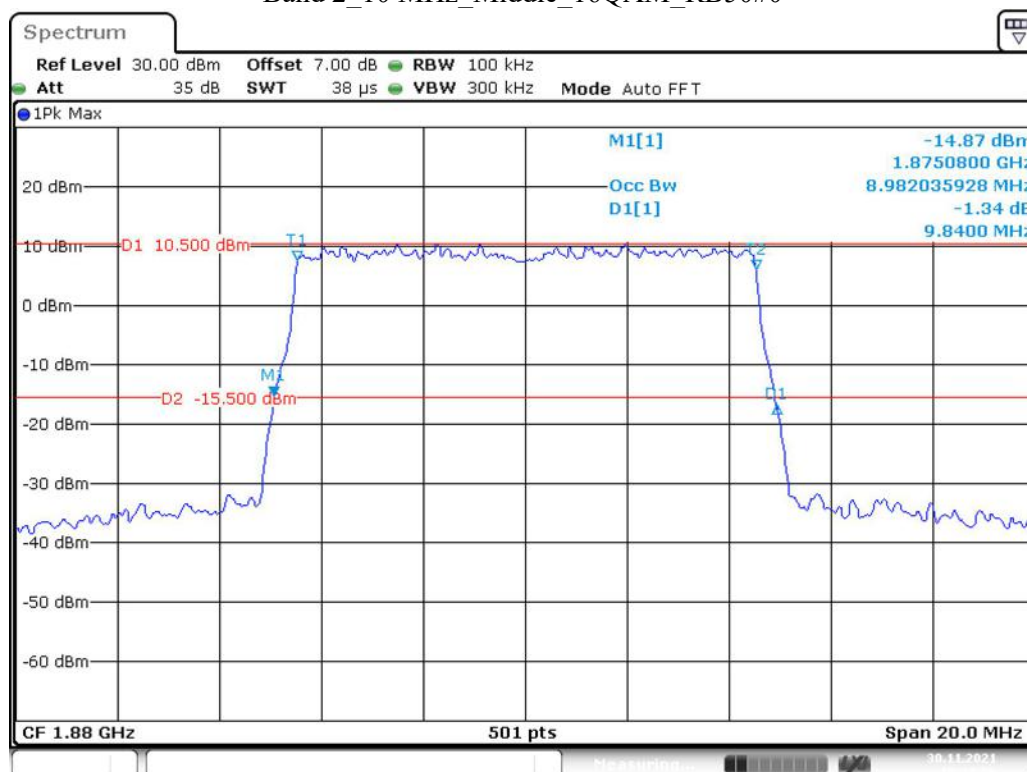
Band 2 10 MHz Middle 16QAM RB50#0
