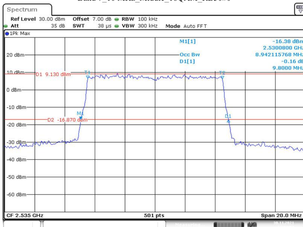
Band 7 10 MHz Middle 16QAM RB50#0
