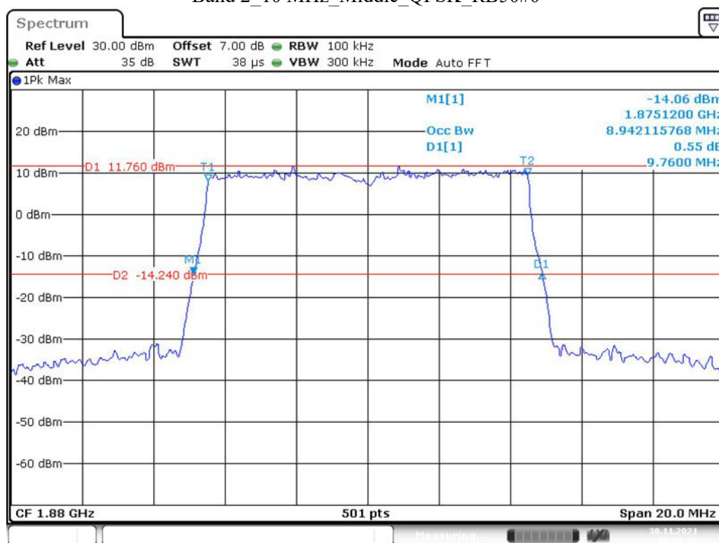
Band 2 10 MHz Middle QPSK RB50#0
