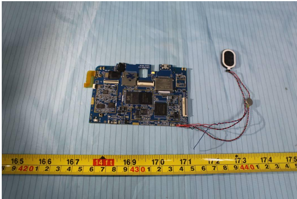
EUT – Main Board Top Shielding off View
