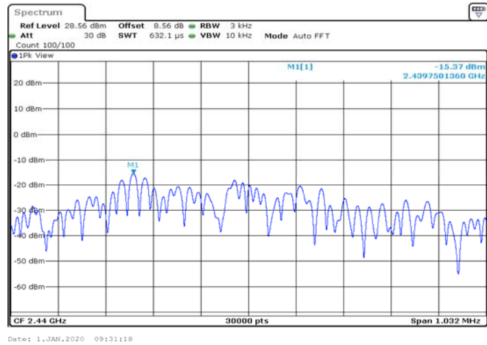
BLE_BT4.0_Ant1_2440
