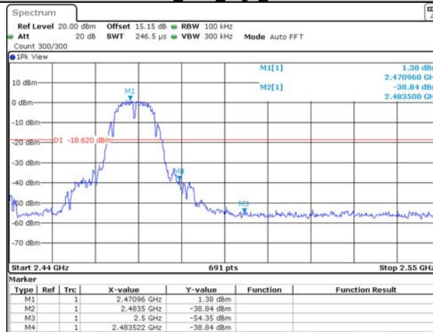
11B_Ant1_High_2472
