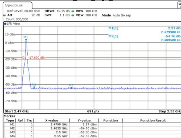
DH1_Ant1_High_2480
