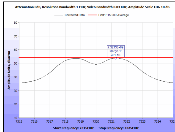
Plot 38. Radiated Emissions, Average, Mid Channel, CF 2440MHz, 3rd harmonic, 3 wire dimmer
