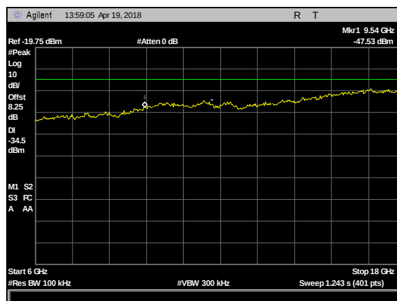
Plot 96. 100 kHz Spurious Emissions, high channel, CF 2480M, 6-18GHz
