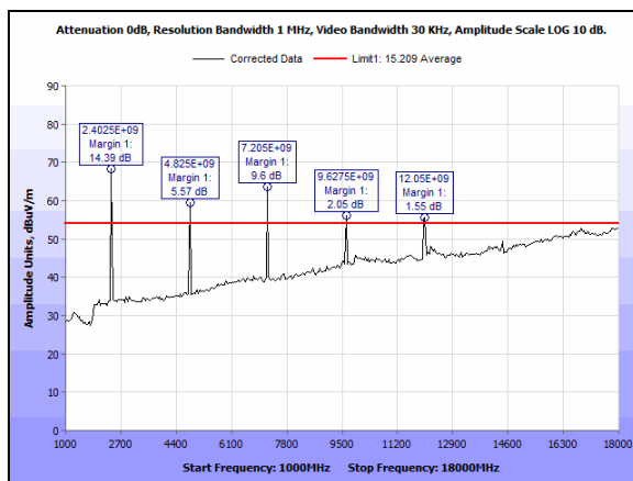
Plot 63. Radiated Emissions, Average, Low Channel, 2405M, 1-18GHz, Switch
