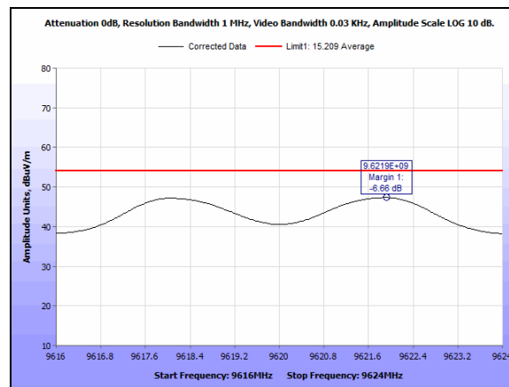
Plot 66. Radiated Emissions, Average, Low Channel, 2405M, 1-18GHz, 4th Harmonic, Switch
