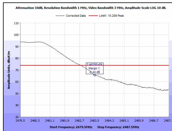
Plot 87. Radiated Restricted Band Edge, High Channel, Peak, CF 2480M, KEYPAD
