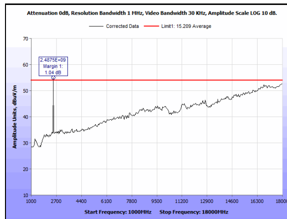
Plot 17. Radiated Emissions, Average, high channel, 2480M, 1-18GHz - 2w dimmer
