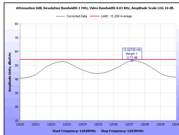
Plot 21. Radiated Emissions, Average, low channel, 2405M, 1-18GHz, 5th harmonic - 2w dimmer
