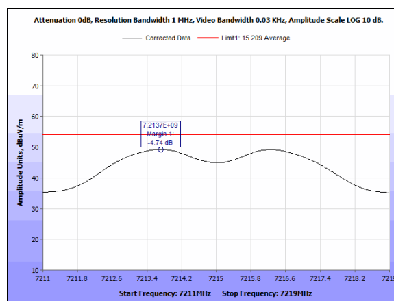
Plot 19. Radiated Emissions, Average, low channel, 2405M, 1-18GHz, 3rd harmonic - 2w dimmer
