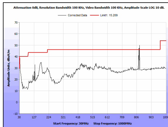
Plot 45. Radiated Emissions, Low Channel, 2405M, 0.03-1GHz - 3w dimmer
