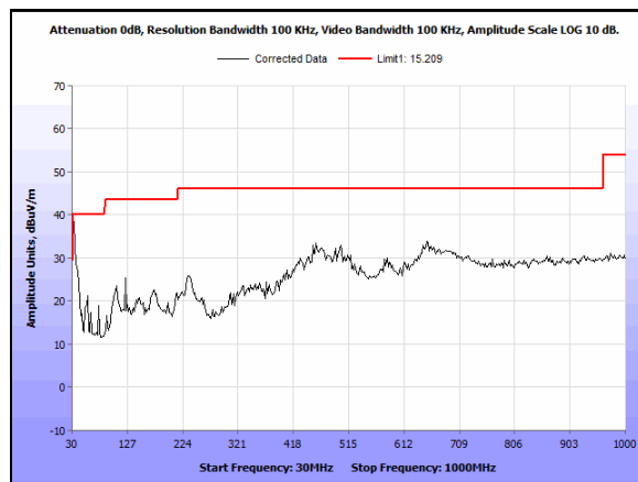
Plot 76. Radiated Emissions, Mid Channel, 2440M, 0.03-1GHz - Switch
