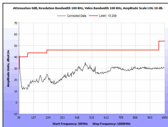
Plot 75. Radiated Emissions, Low Channel, 2405M, 0.03-1GHz - Switch
