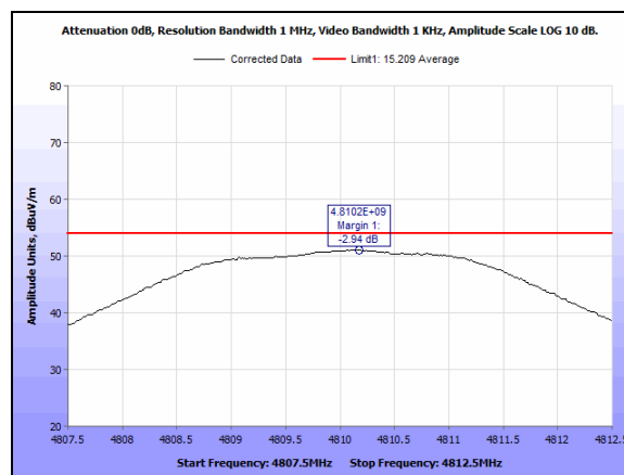
Plot 33. Radiated Emissions, Average, Low Channel, CF 2405MHz, 2nd harmonic, 3 wire dimmer
