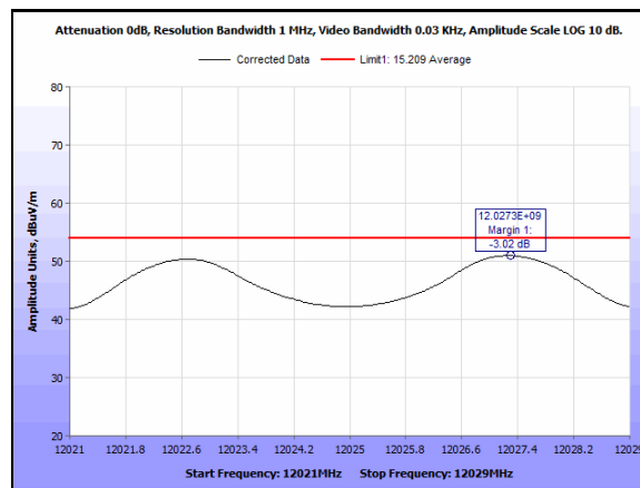
Plot 67. Radiated Emissions, Average, Low Channel, 2405M, 1-18GHz, 5th Harmonic, Switch
