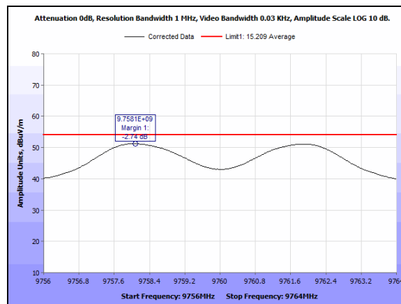
Plot 54. Radiated Emissions, Average, Mid Channel, 2440M, 1-18GHz, 4th Harmonic - Keypad
