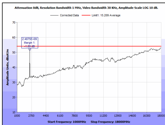
Plot 62. Radiated Emissions, Average, High Channel, 2480M, 1-18GHz, Lowest Setting, Switch
