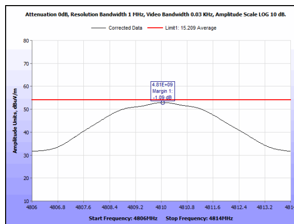
Plot 49. Radiated Emissions, Average, Low Channel, 2405M, 1-18GHz, 2nd Harmonic - Keypad
