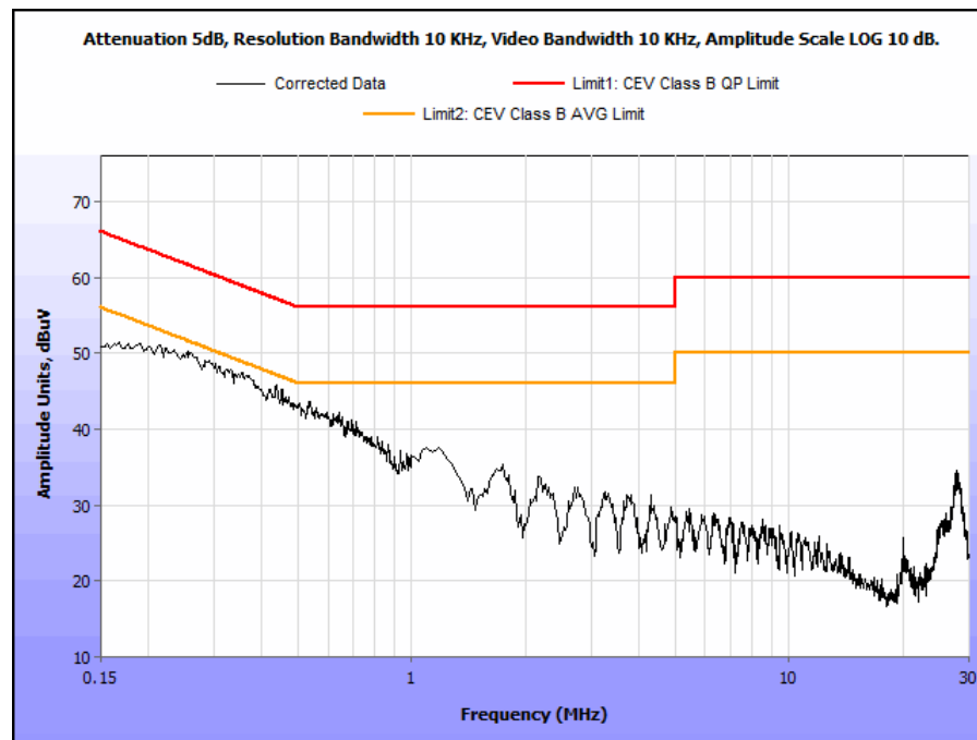
Plot 8. Conducted Emissions, 15.207(a), Standard Switch, Neutral Line
