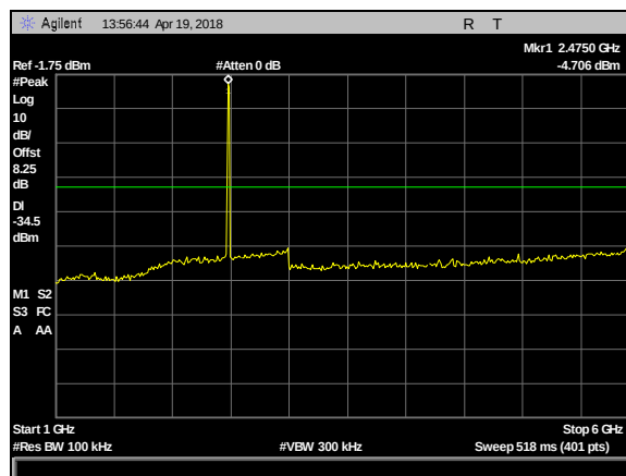
Plot 95. 100 kHz Spurious Emissions, high channel, CF 2480M, 1-6GHz
