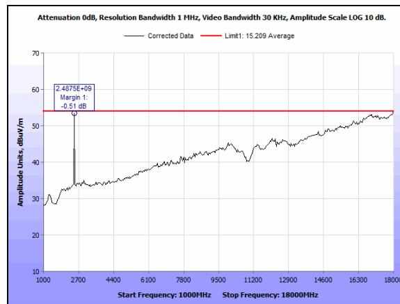
Plot 47. Radiated Emissions, Average, High Channel, 2480M, 1-18GHz - keypad
