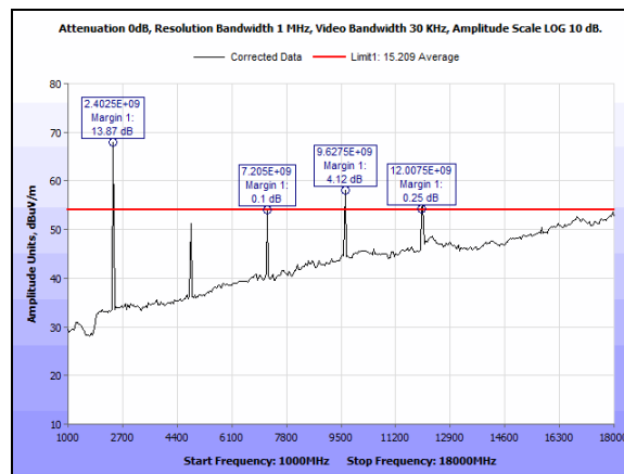
Plot 18. Radiated Emissions, Average, low channel, 2405M, 1-18GHz - 2w dimmer
