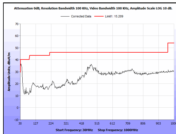
Plot 61. Radiated Emissions, Mid Channel, 2440M, 0.03-1GHz - Keypad
