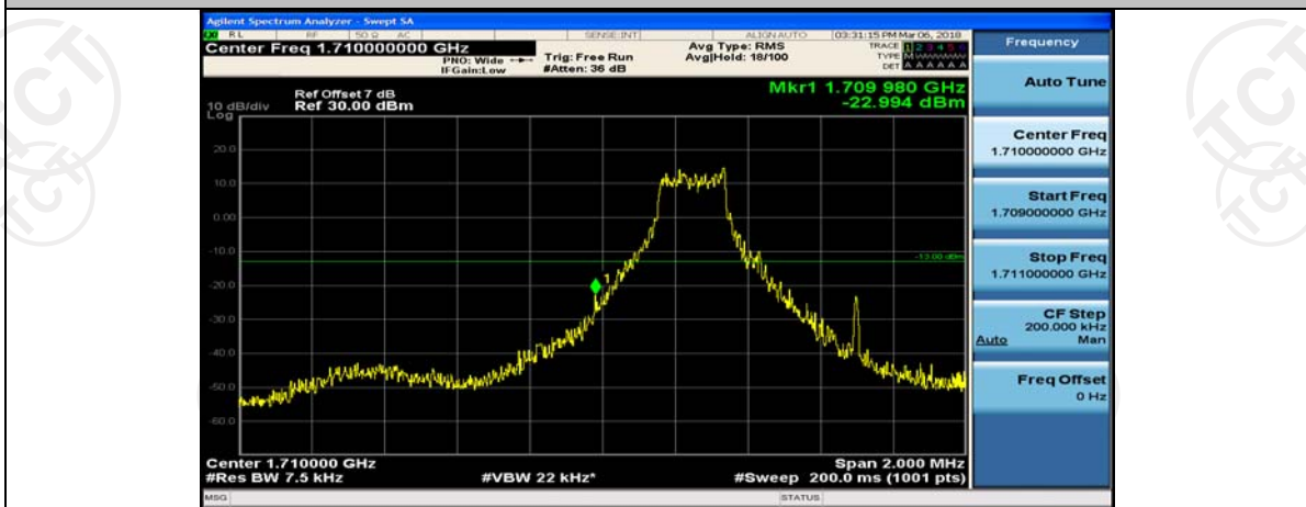
(Channel Bandwidth: 1.4 MHz)_LCH_16QAM_1RB#3
