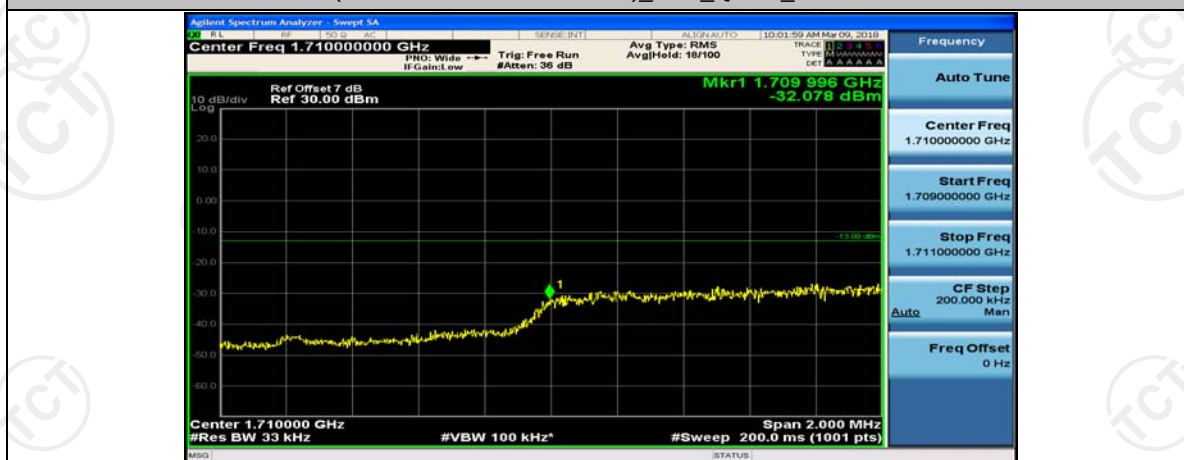
(Channel Bandwidth: 3 MHz)_LCH_QPSK_15RB#0
