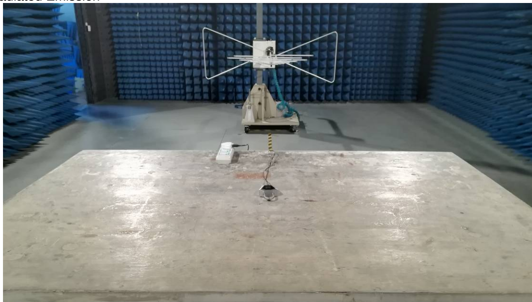
Radiated Emission
