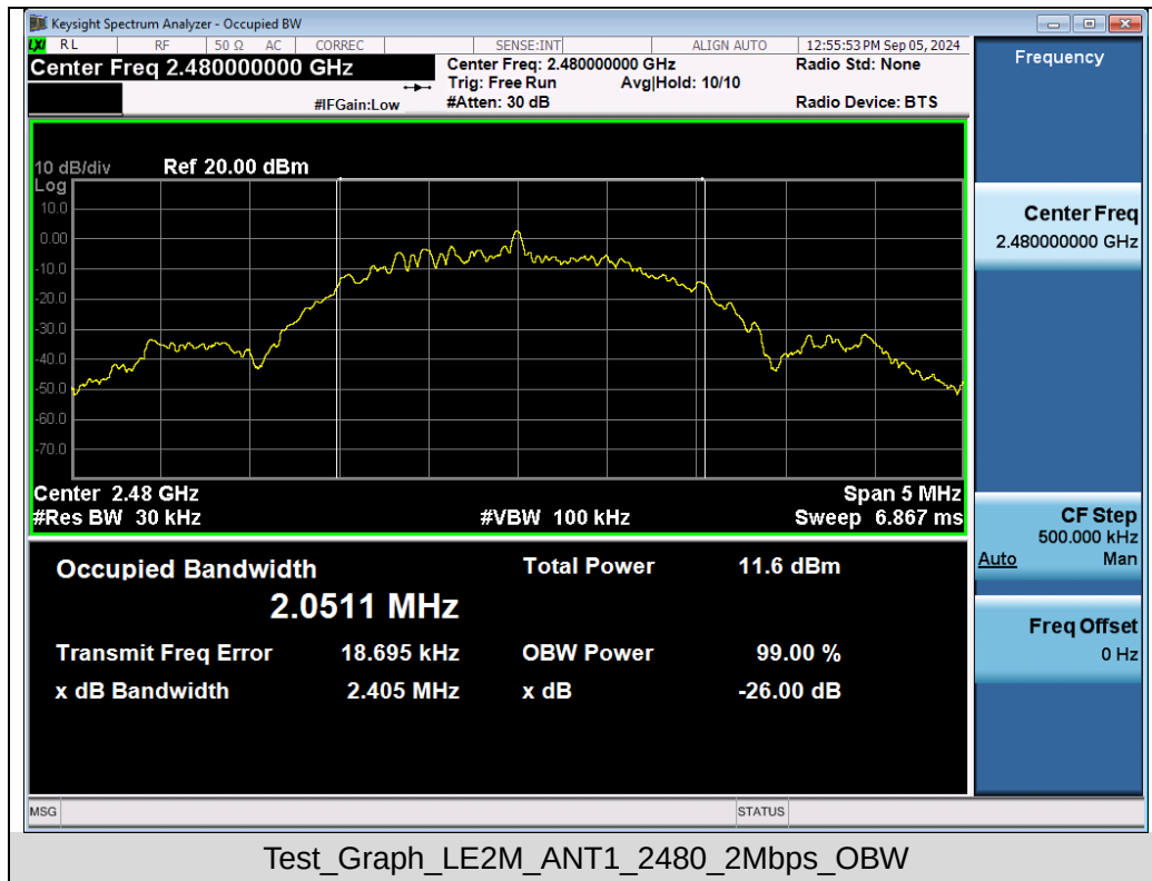
Test Graphs of DTS Bandwidth
