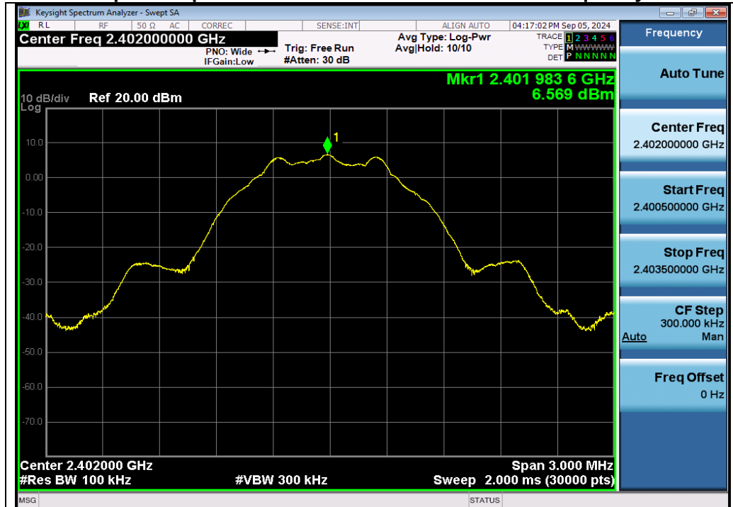
Test_Graph_LE1M_ANT1_2402_1Mbps_Reference Level
