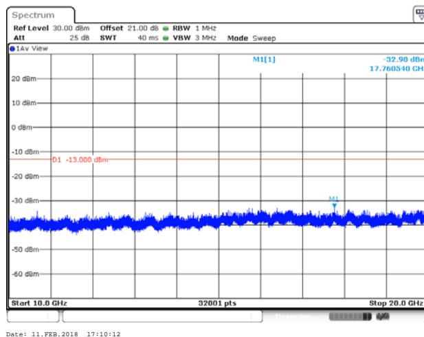
CH 1413 10GHz – 20GHz
