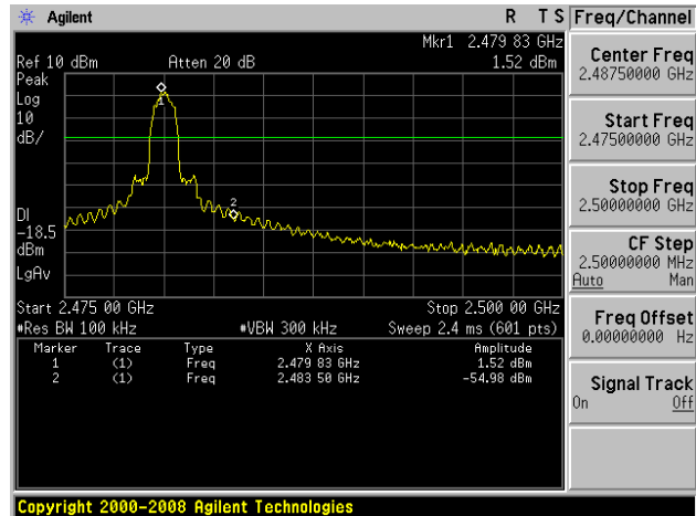
8-DPSK: Band Edge-High Channel
