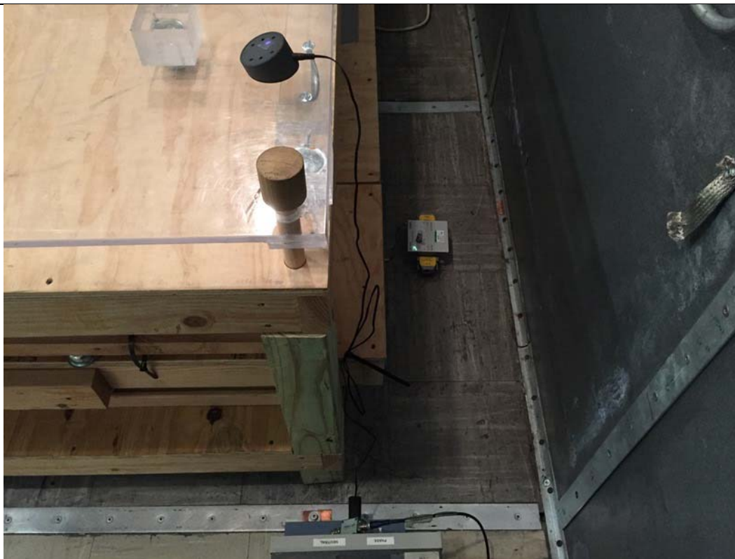
Conducted Mains Emissions; View 2
