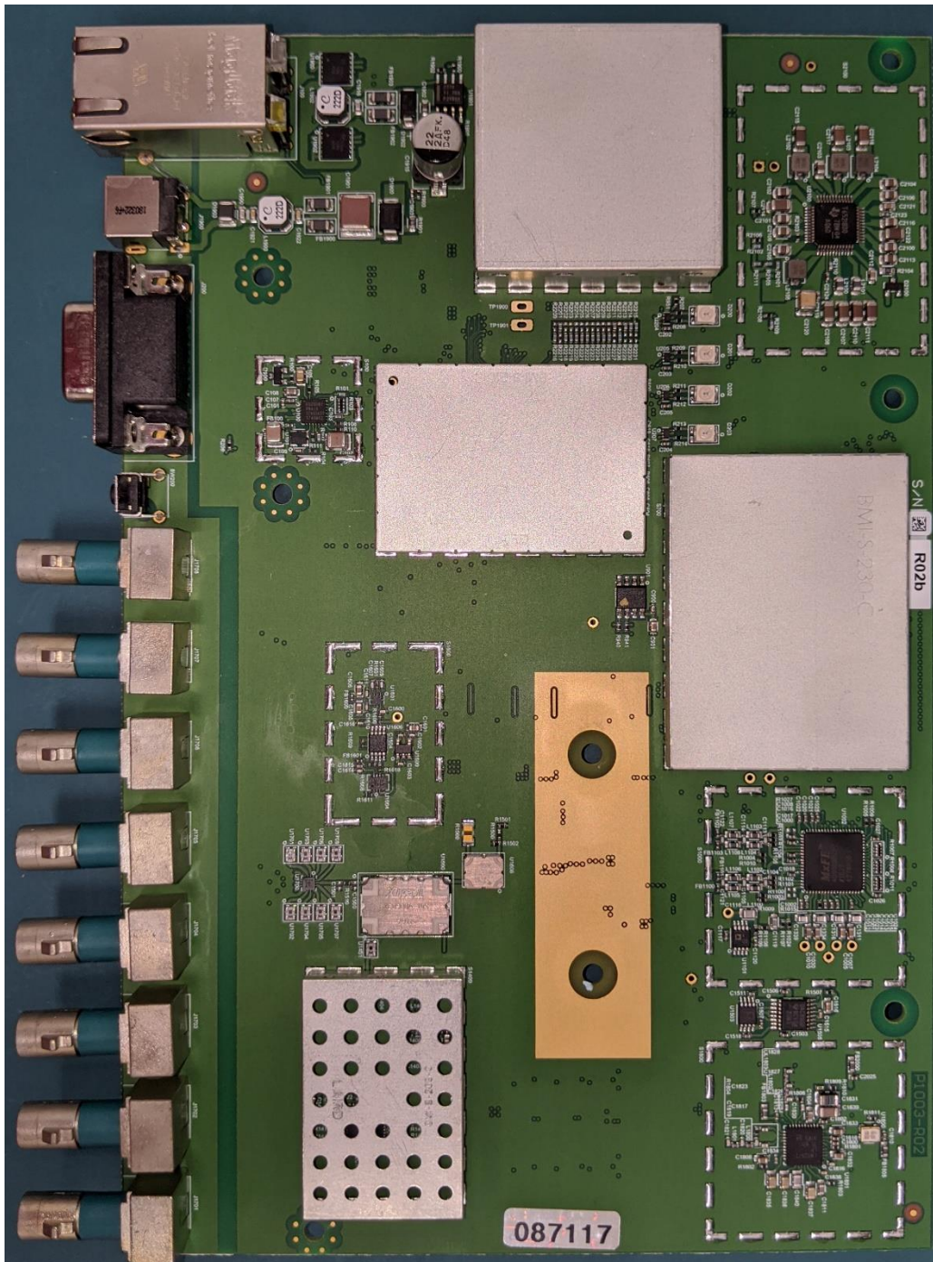
Figure 1: Top Side, Shield Can Lids Installed
