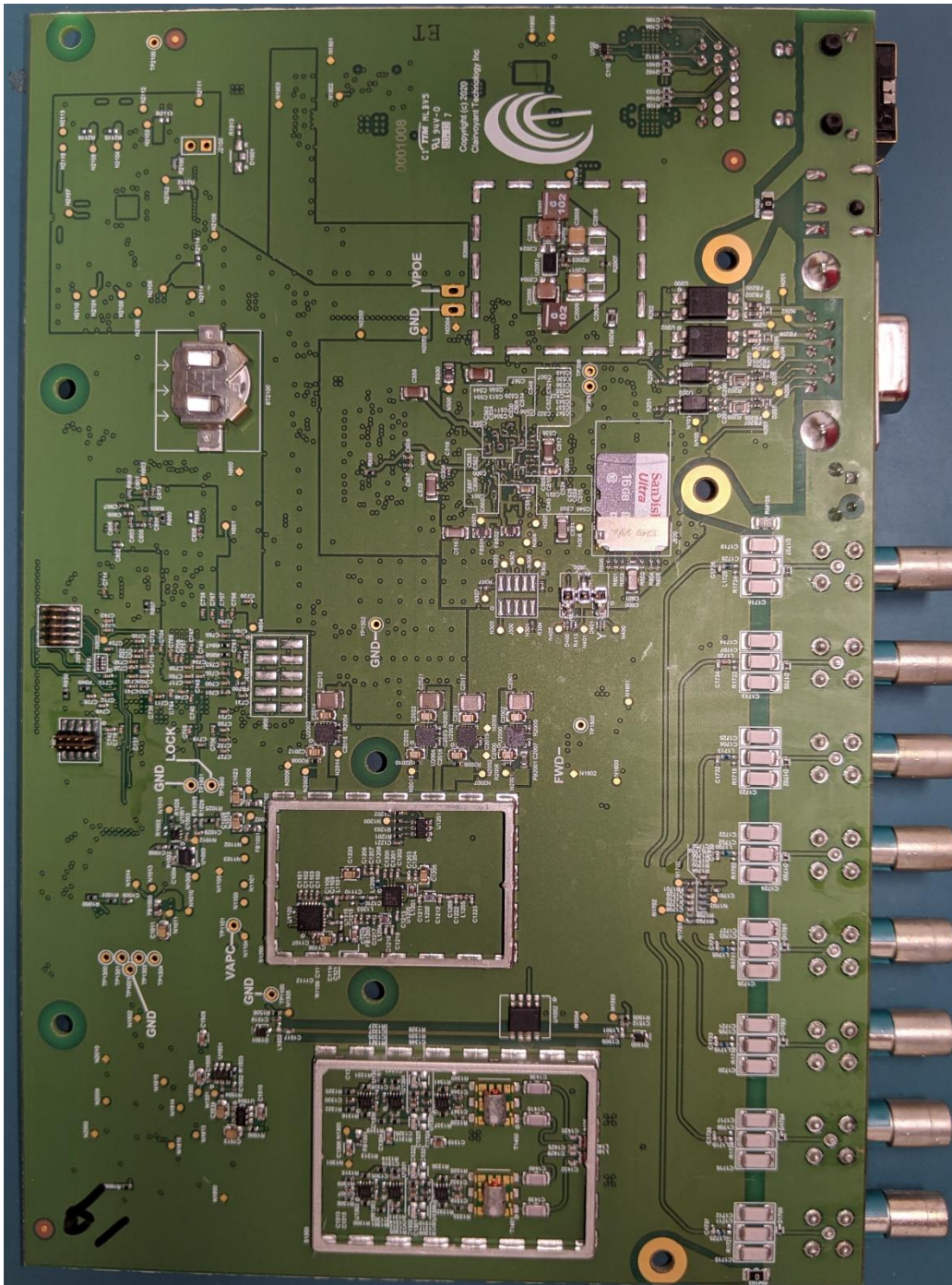
Figure 4: Bottom Side, Shield Can Lids Removed
