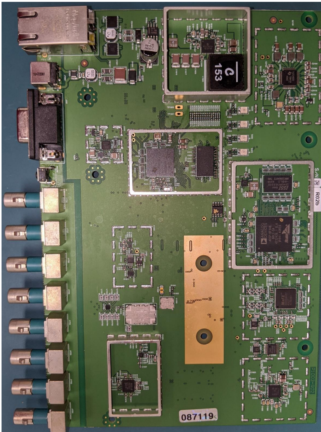
Figure 2: Top Side, Shield Can Lids Removed
