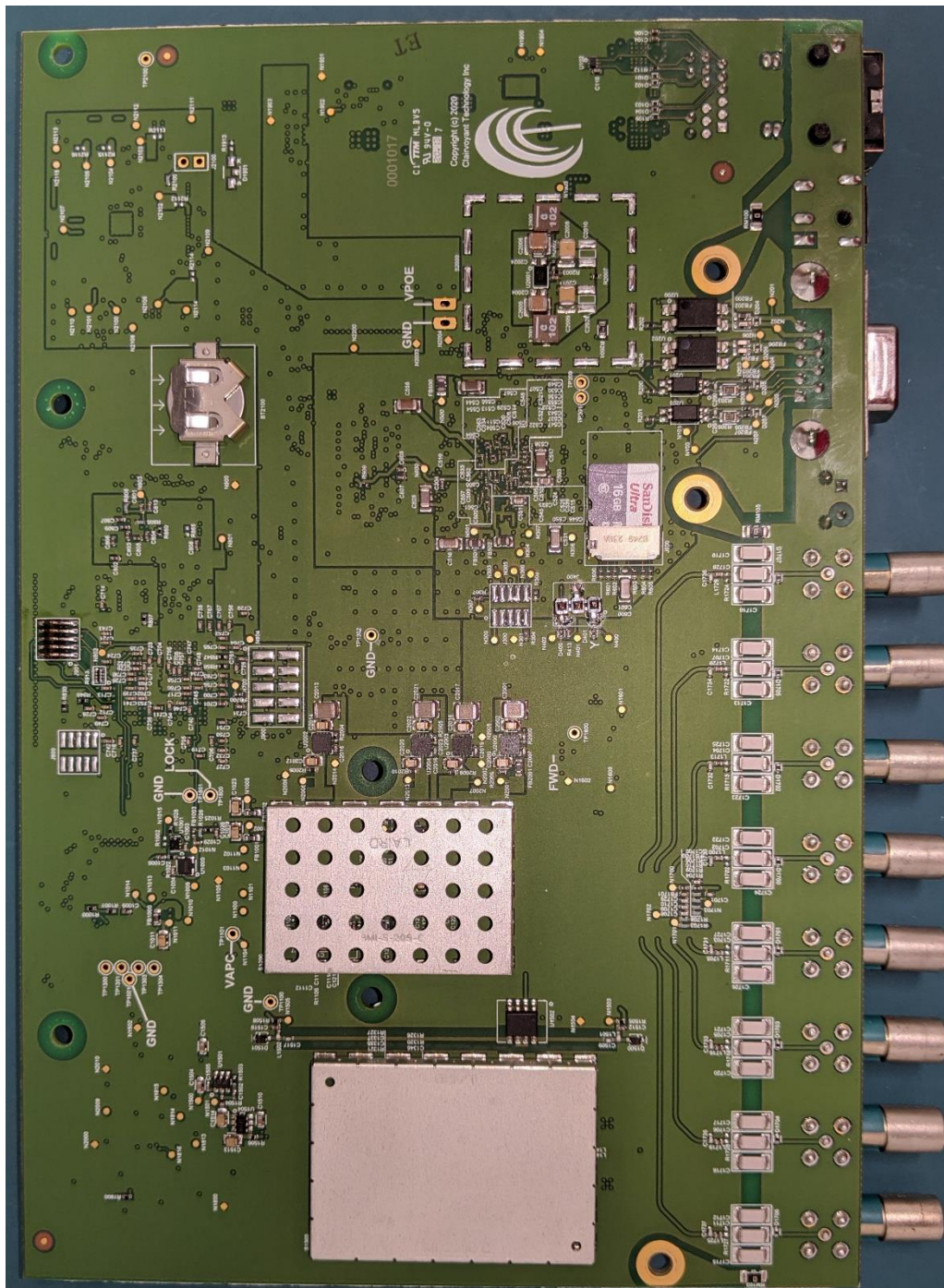
Figure 3: Bottom Side, Shield Can Lids Installed
