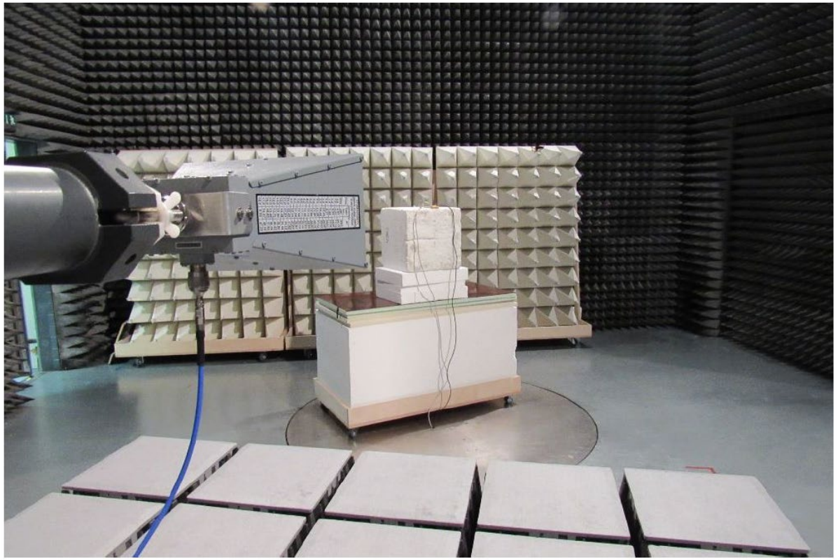
VIEW C
