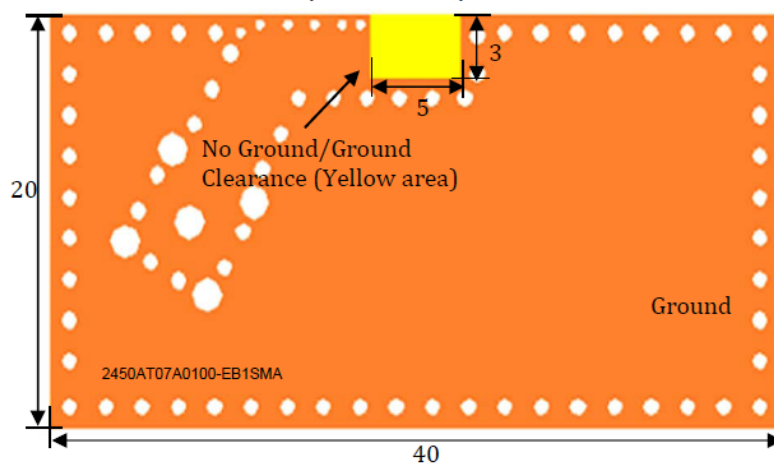
Test Board-Bottom View (Units in mm)
