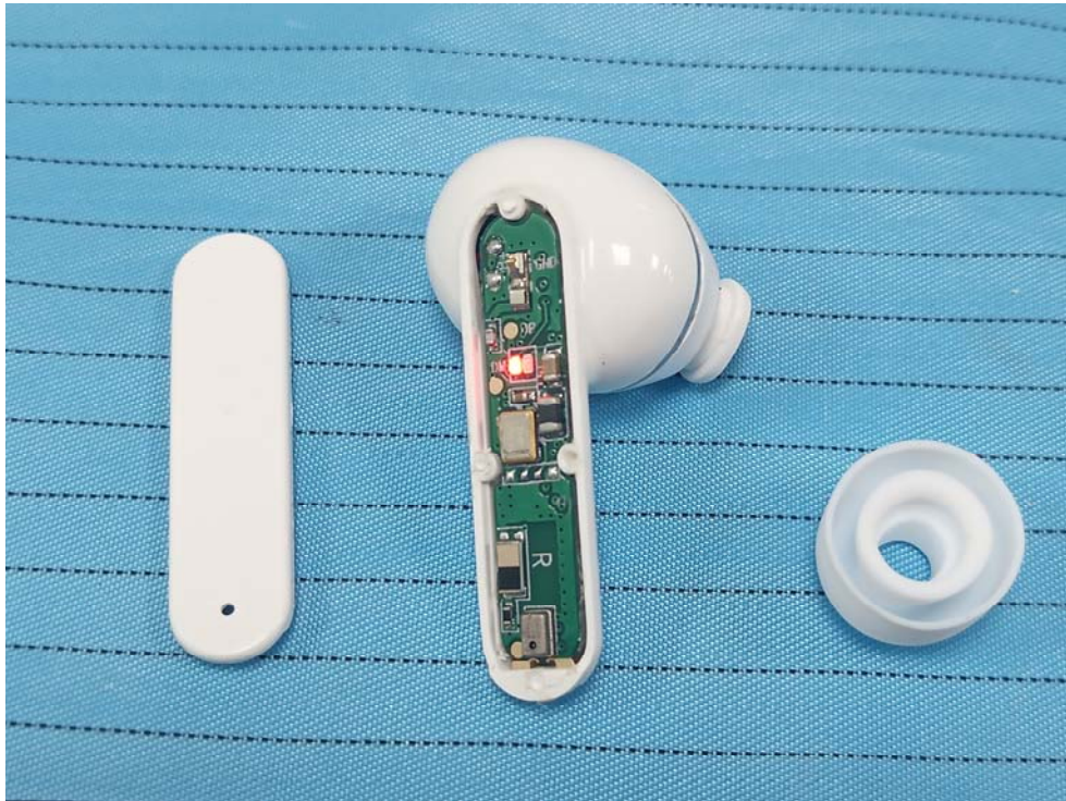
Right earphone
