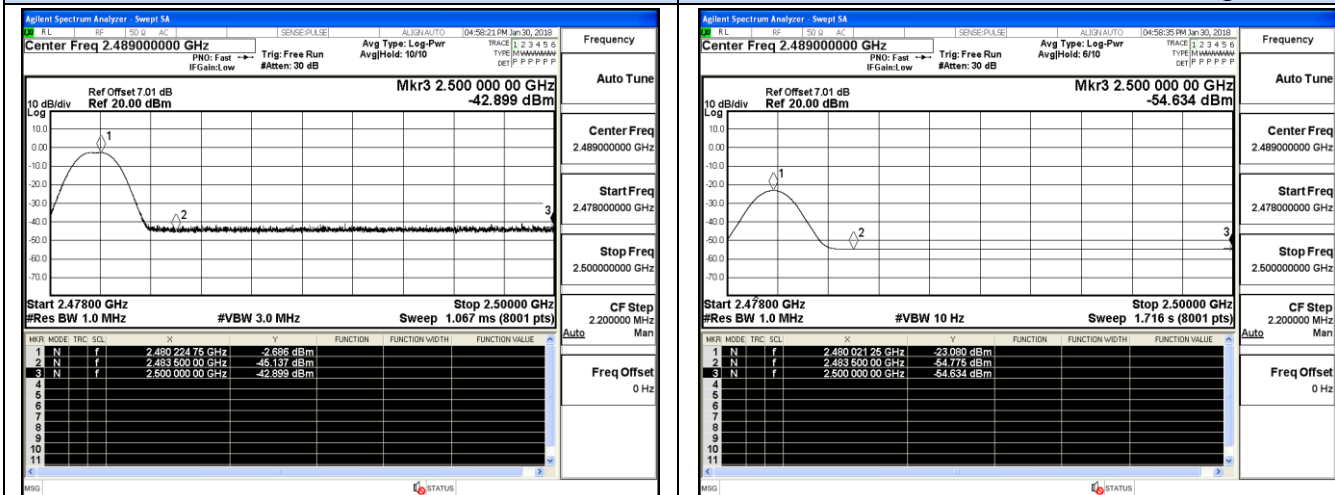
Channel 39 / 2480 MHz – Average
