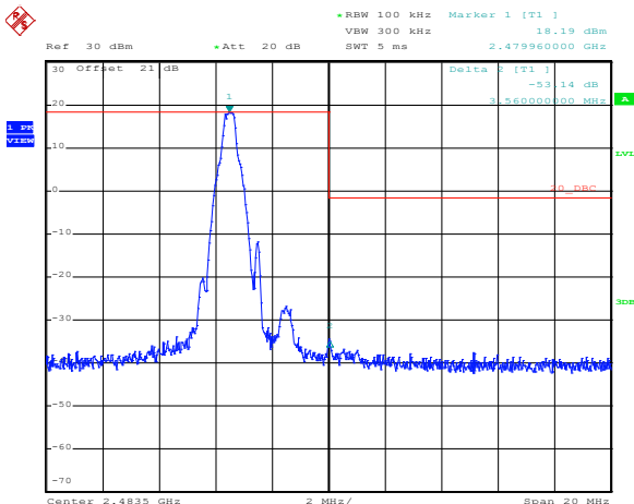
Figure 8.5-6: Conducted spurious emissions at the upper band edge, Tx-2480 MHz
