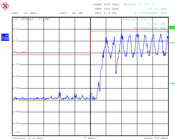
Figure 8.5-7: Conducted spurious emissions at the lower band edge, Hopping
