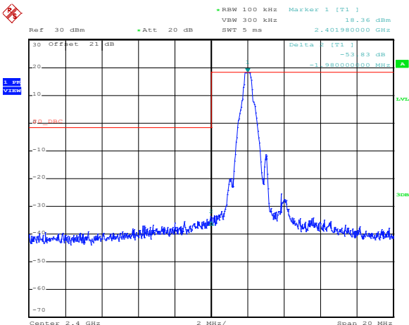
Figure 8.5-5: Conducted spurious emissions at the lower band edge, Tx-2402 MHz
