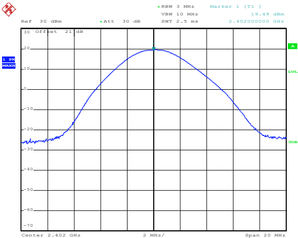
Figure 8.4-1: Peak output power on low channel
