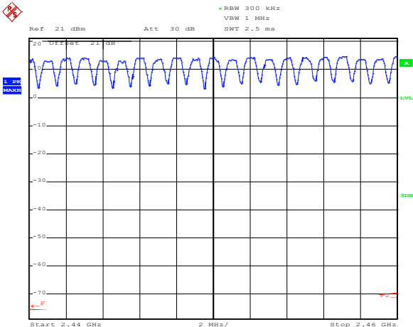
Figure 8.2-7: Number of hopping channels, 2.44 to 2.46 GHz = 20
