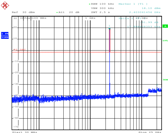
Figure 8.5-1: Conducted spurious emissions, Tx-2402 MHz
