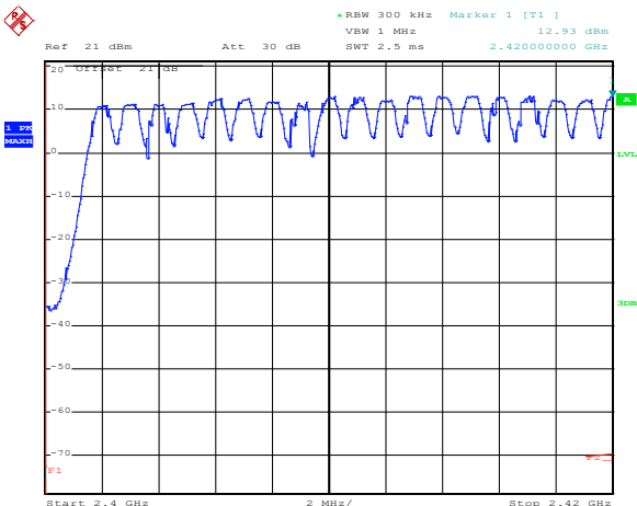
Figure 8.2-5: Number of hopping channels, 2.4 to 2.42 GHz = 18
