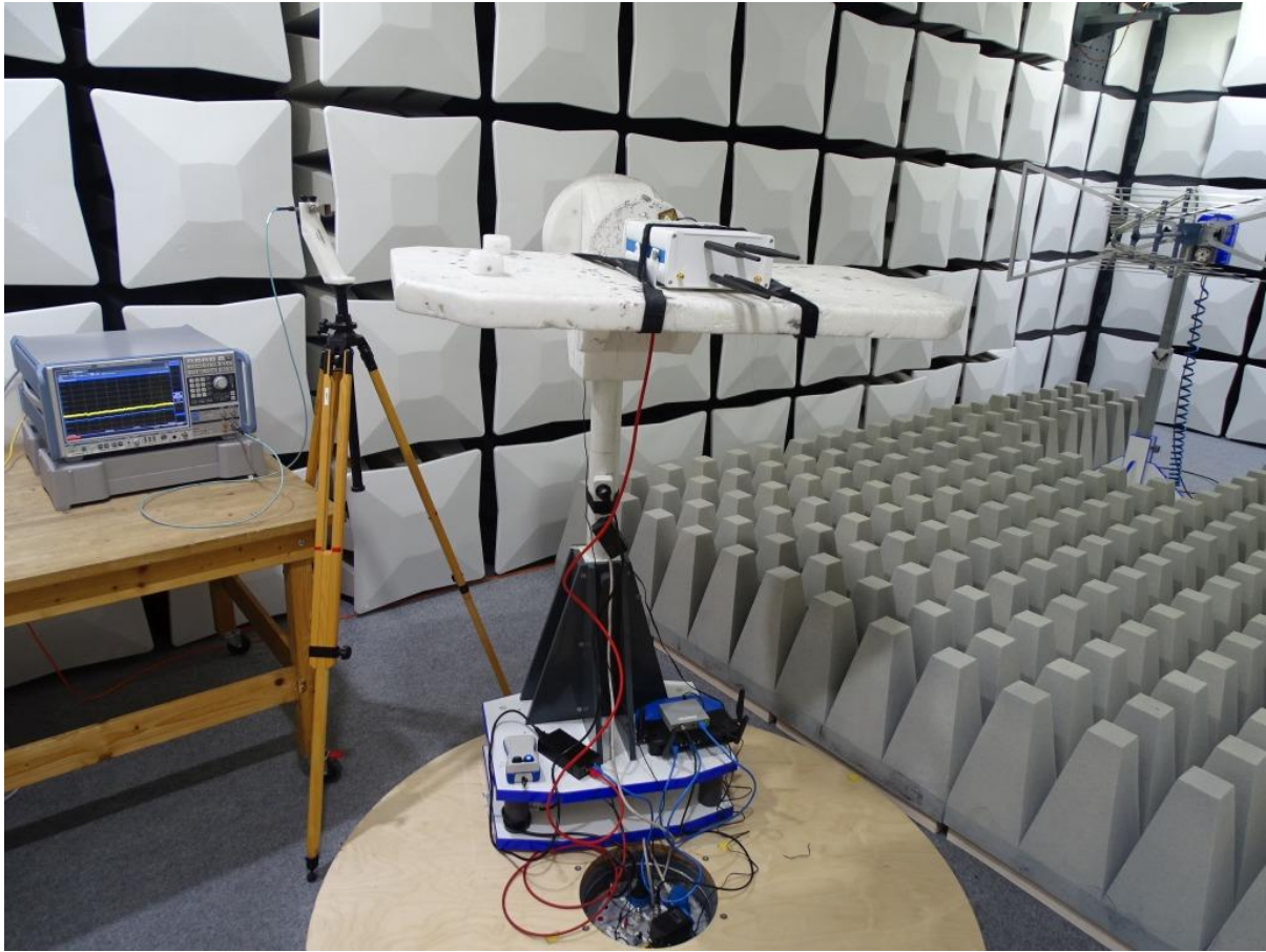
Photo 3: Test setup for radiated measurements above 1 GHz
