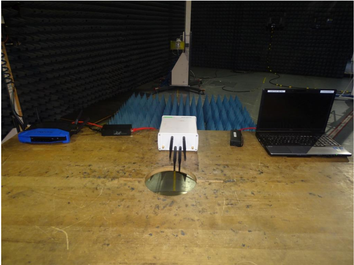
Photo 1: Test setup for radiated measurements starting from 30 MHz
