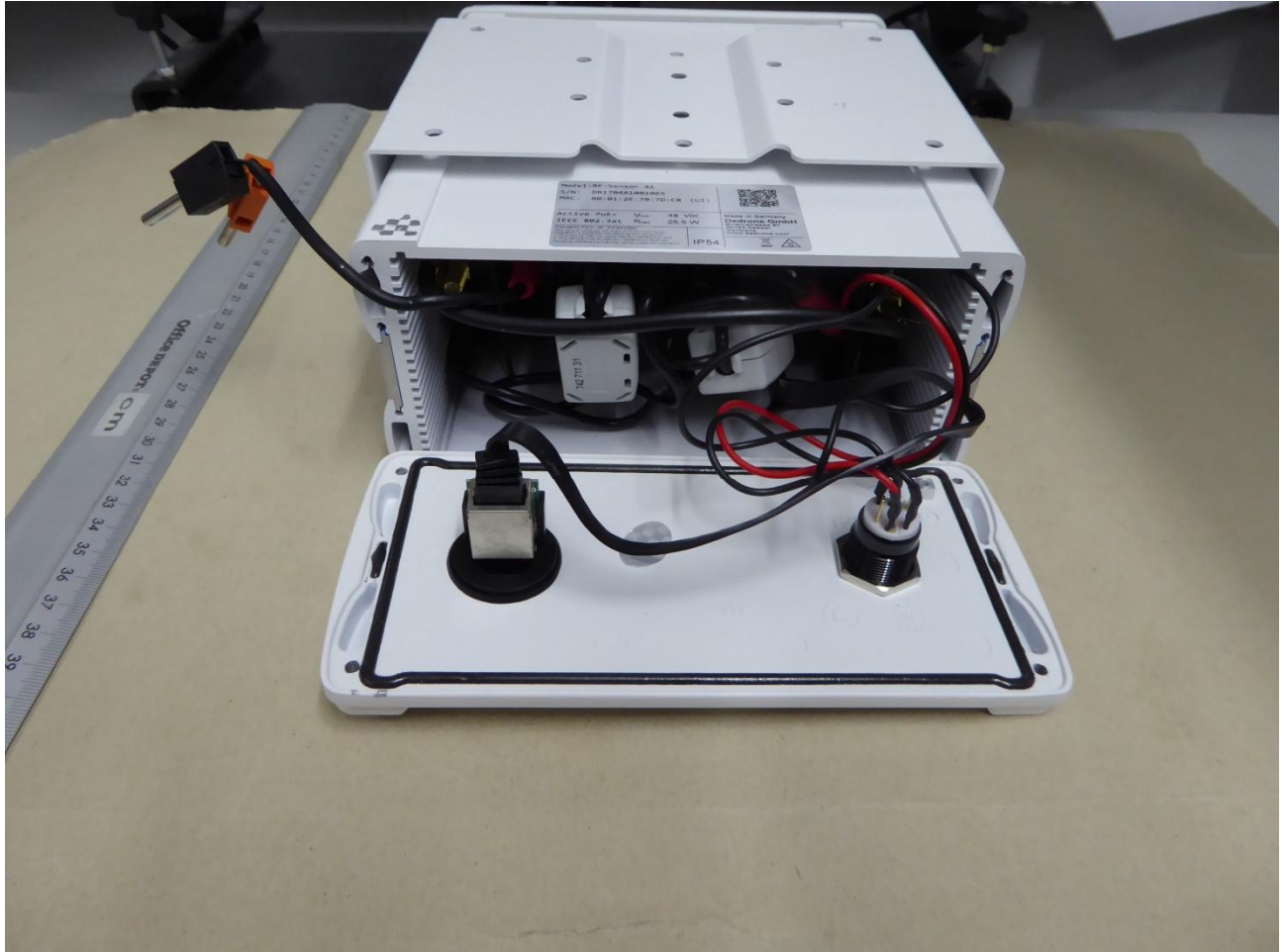
162281_EUT09: EUT bottom view opened
