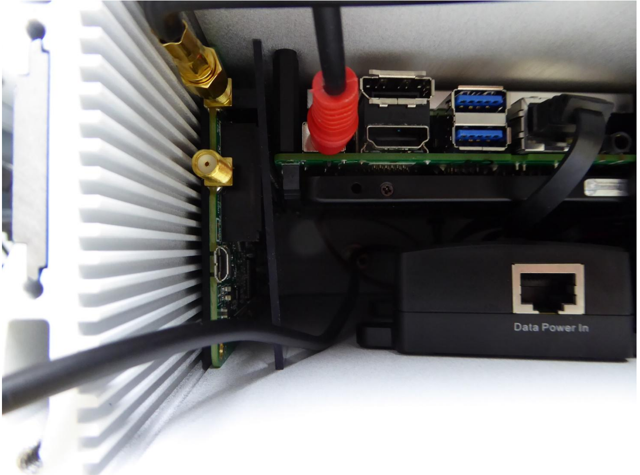
162281_ EUT12: EUT bottom Power/LAN/HackRF detil view
