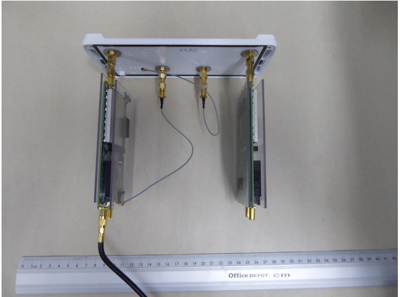
162281_EUT16: EUT 2x HackRF view
