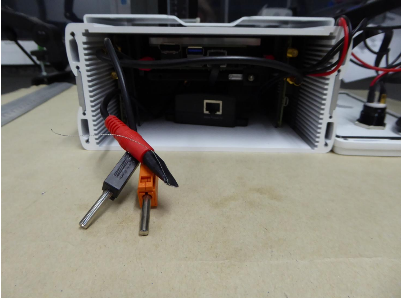
162281_EUT10: EUT bottom view opened
