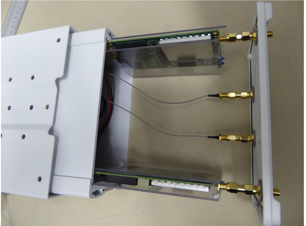
162281_EUT14: EUT internal view
