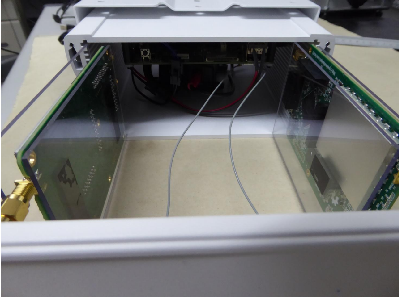
162281_EUT15: EUT internal view
