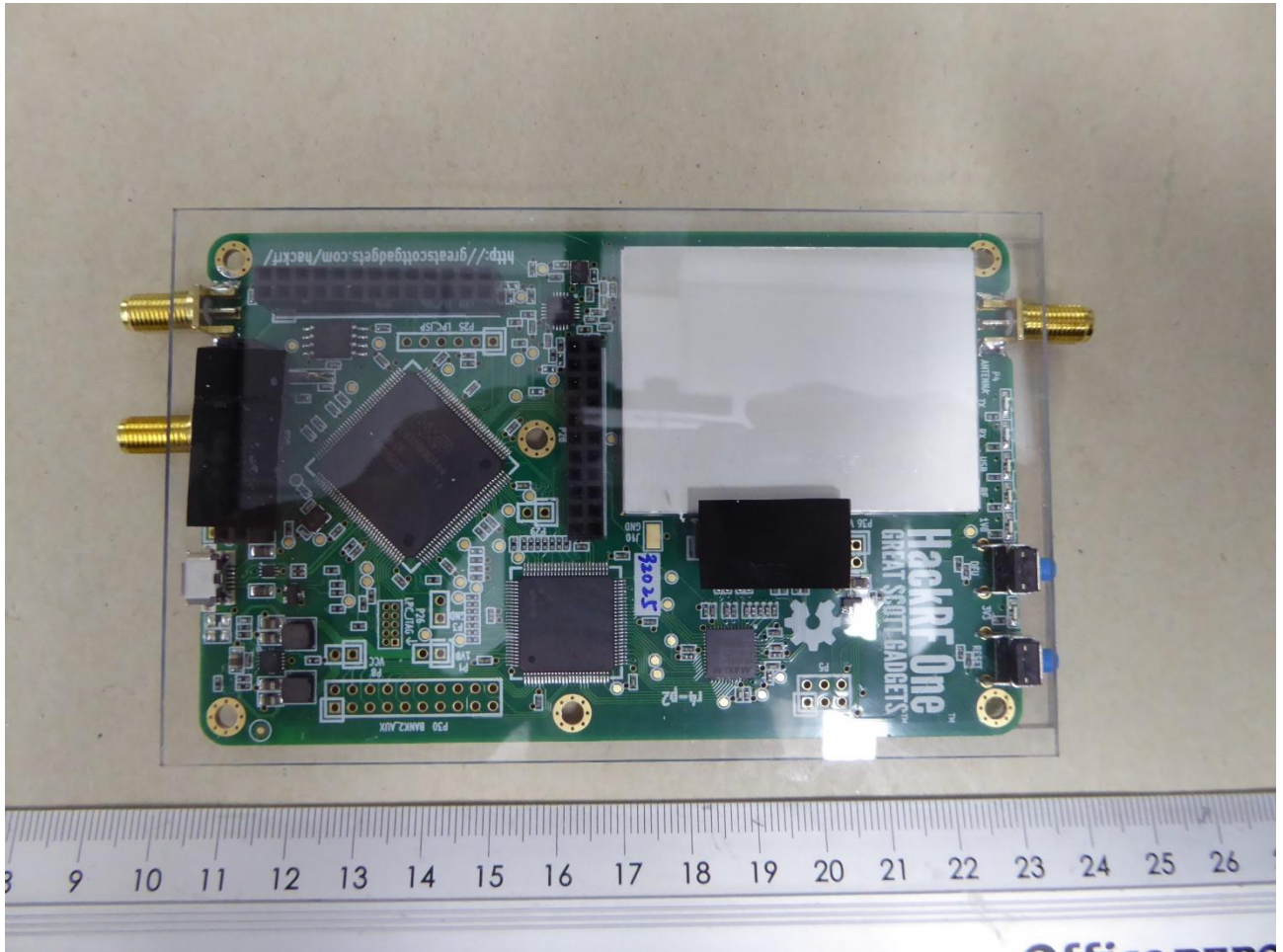
162281_EUT18: HackRF detail view
