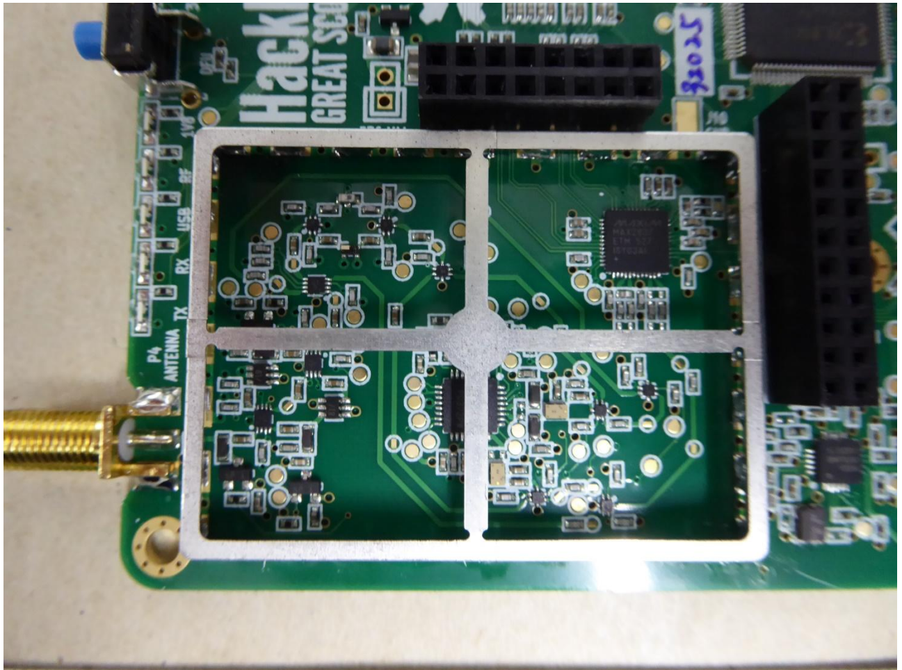
162281_ EUT27: HackRF hf part detail view
