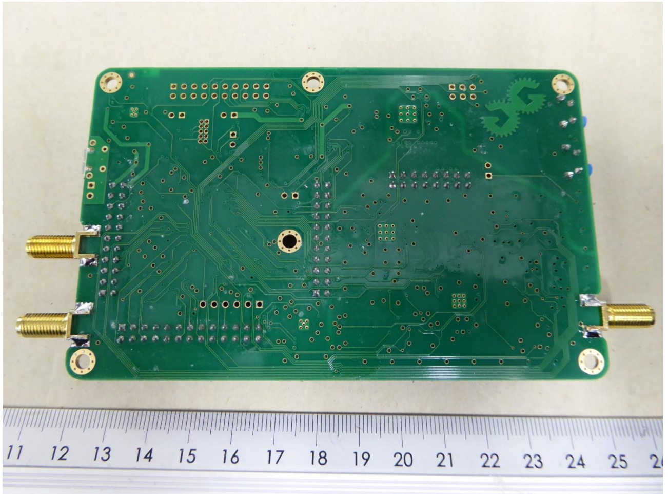
162281_ EUT22: HackRF bottom view
