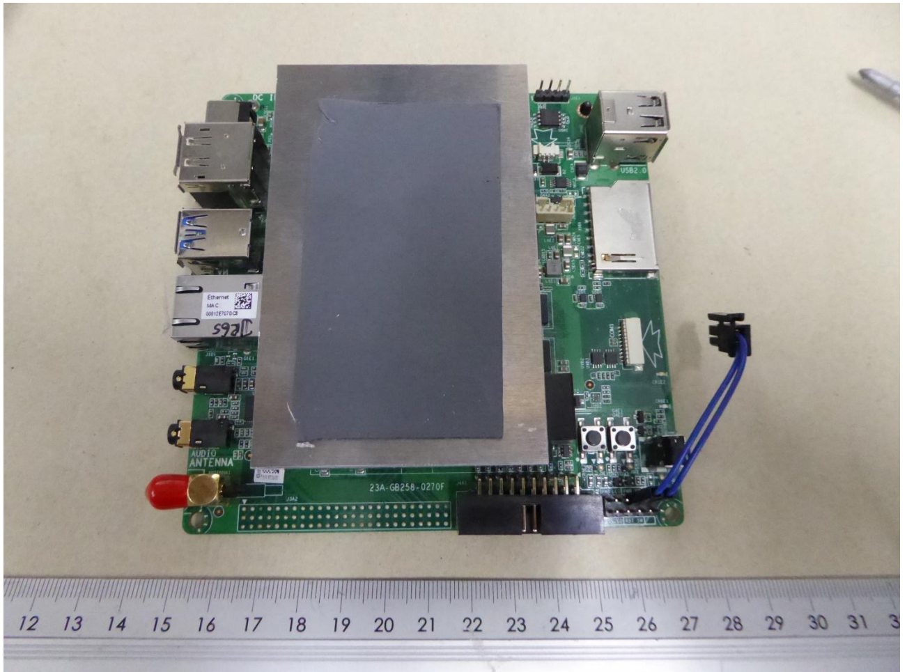
162281_EUT44: Mainboard top view
