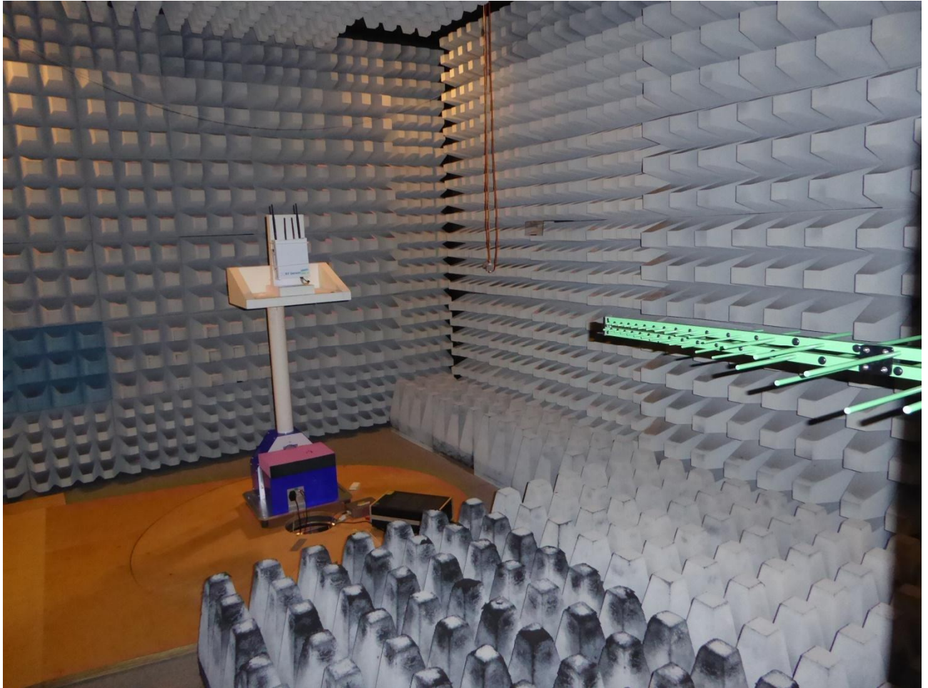
162281_EUT41: Radiated Measurement in the FAR (30MHz – 1GHz)
