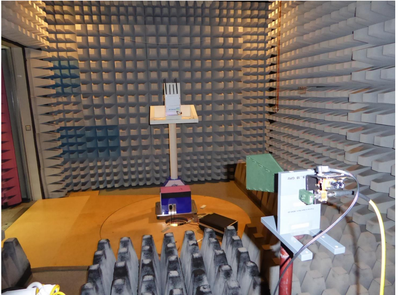
162281_EUT46: Radiated Measurement in the FAR (12 -18 GHz)
