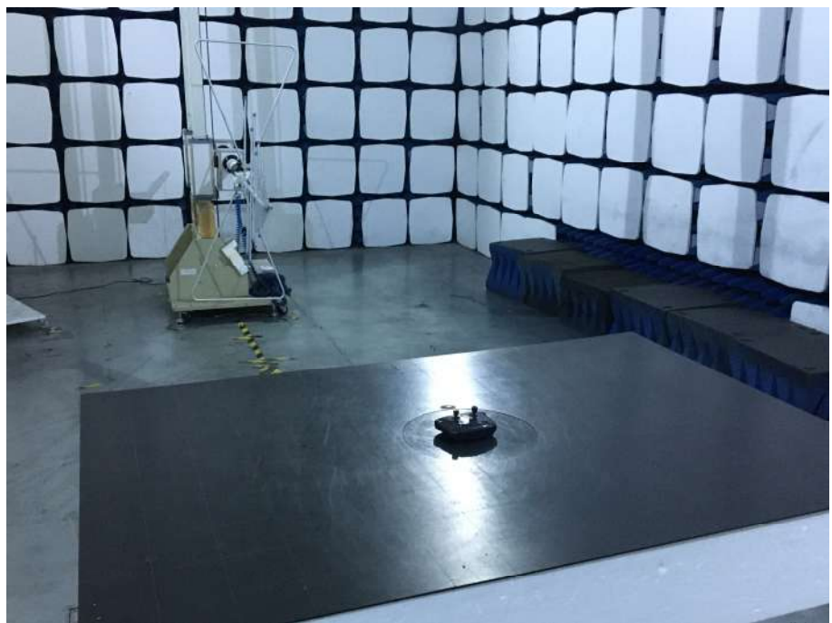
Radiated Emission Test Setup (from 30 MHz to 1 GHz) from 0.8M-Height Turntable Test Table
