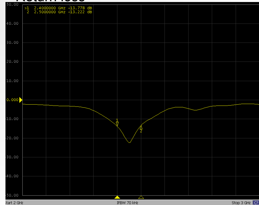
Return loss
