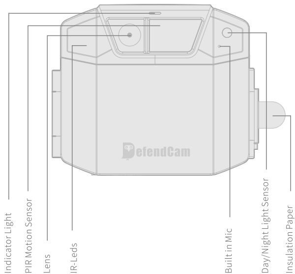
Front View of Camera
