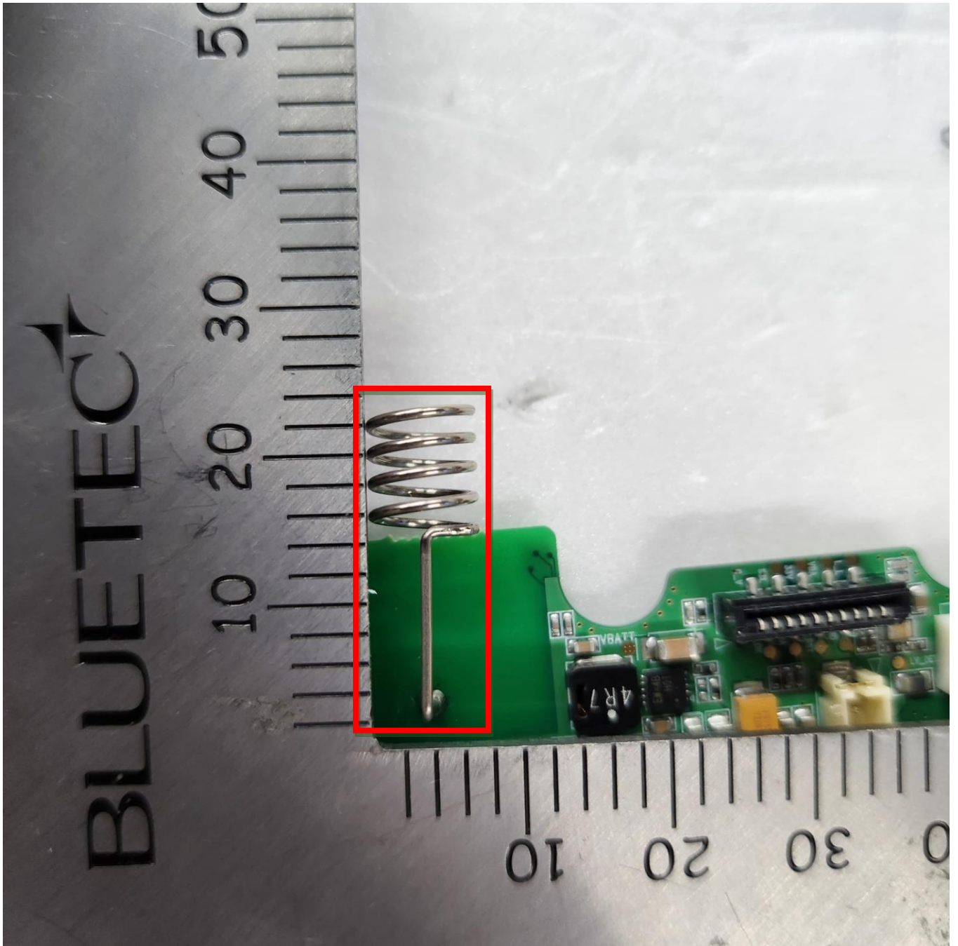
Helical Antenna
